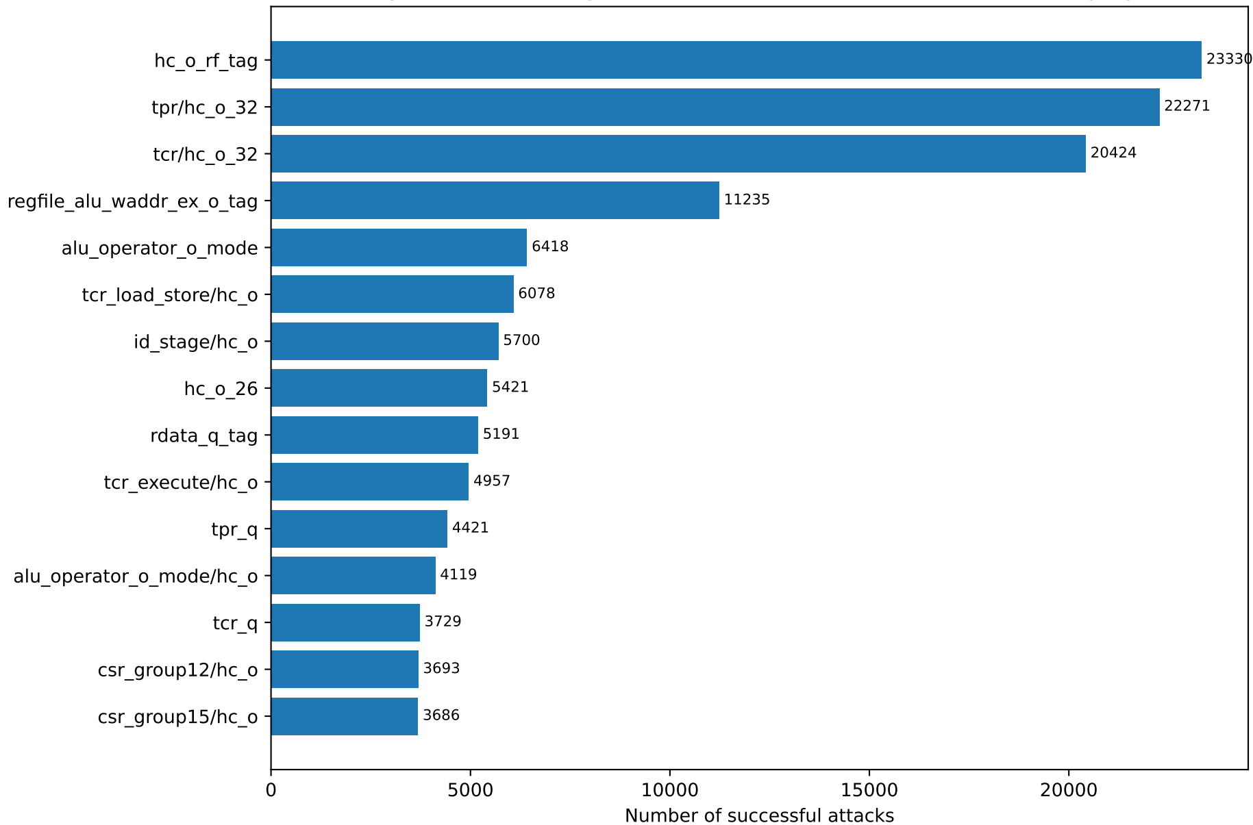
Registers with the highest number of successful attacks — all campaigns
