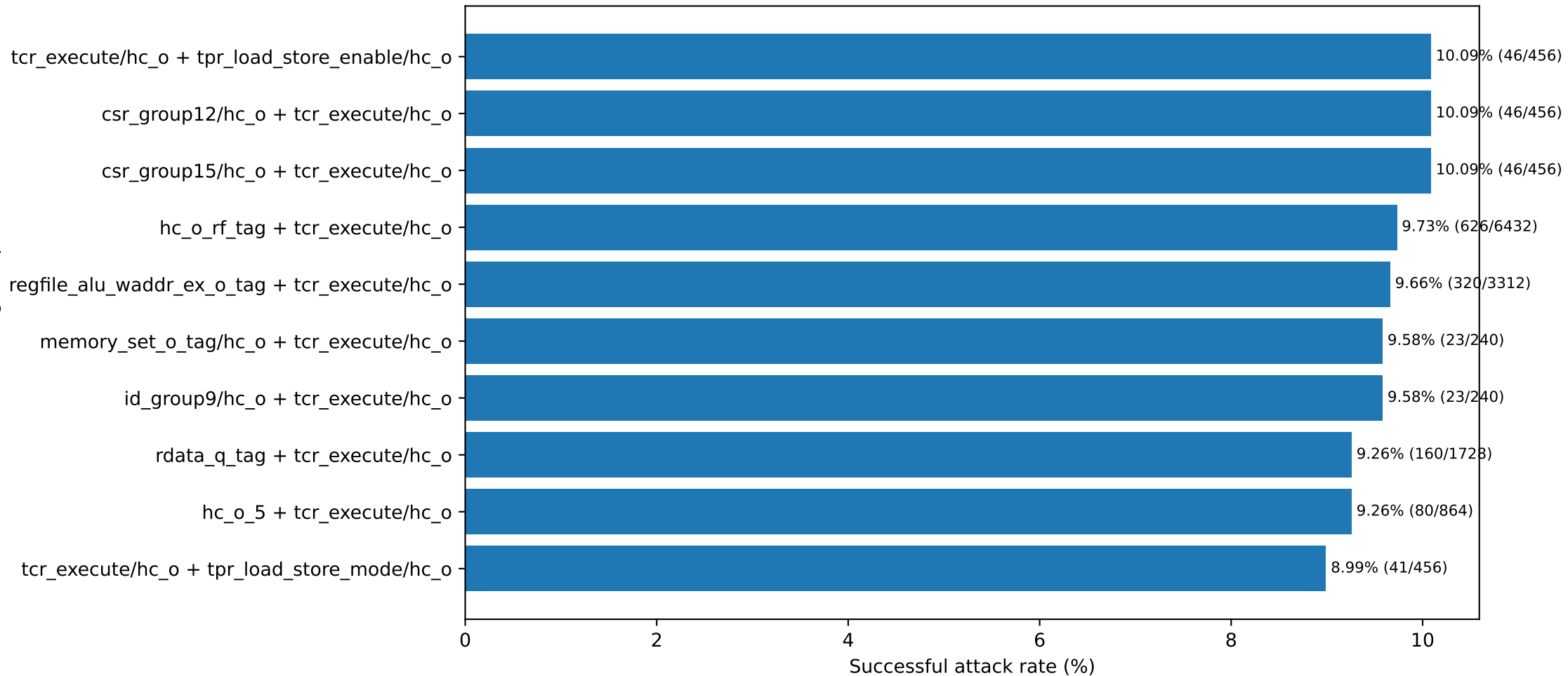
Most vulnerable register pairs — Buffer Overflow
