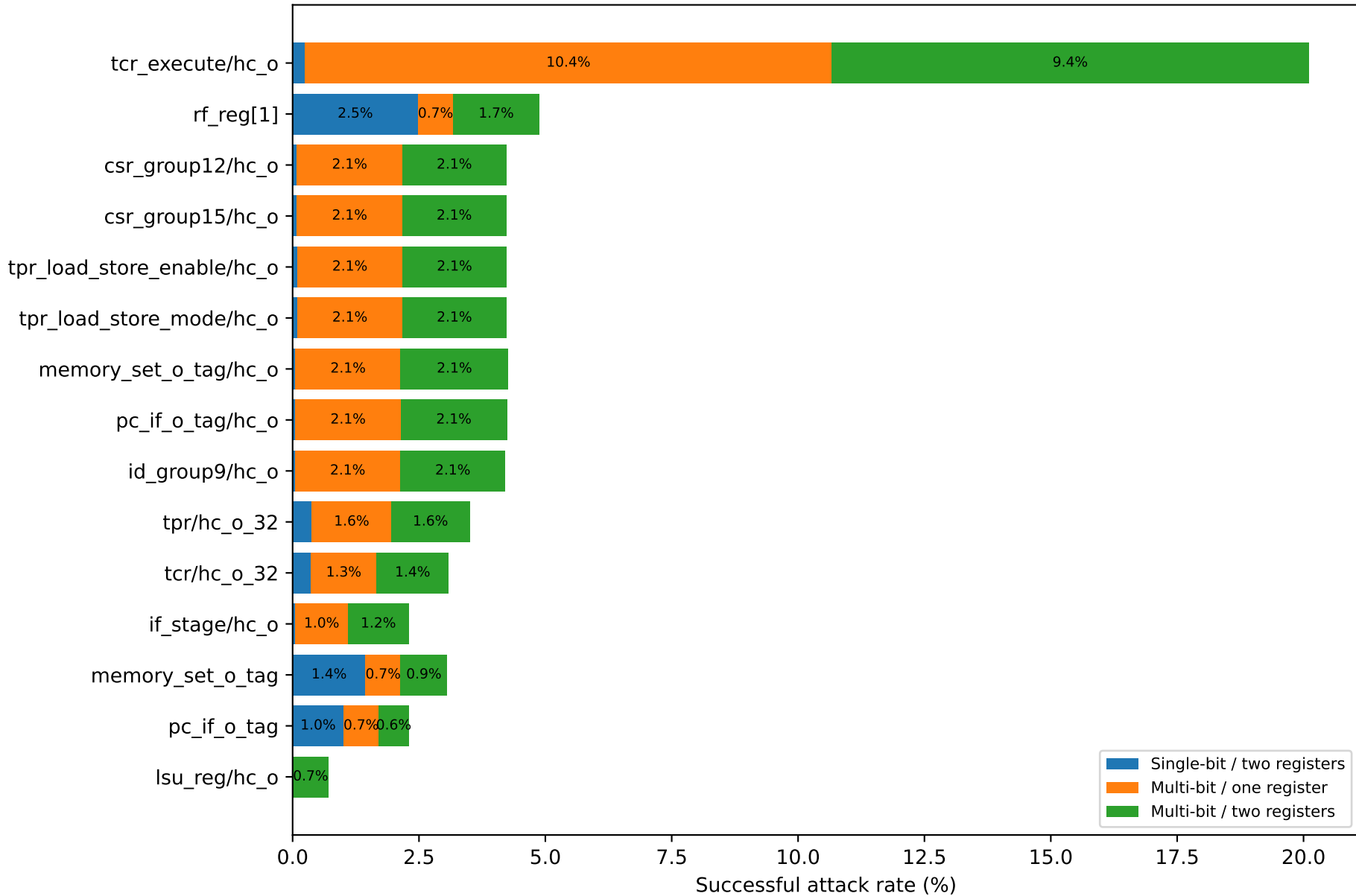
Successful attack rate by fault model — Buffer Overflow
