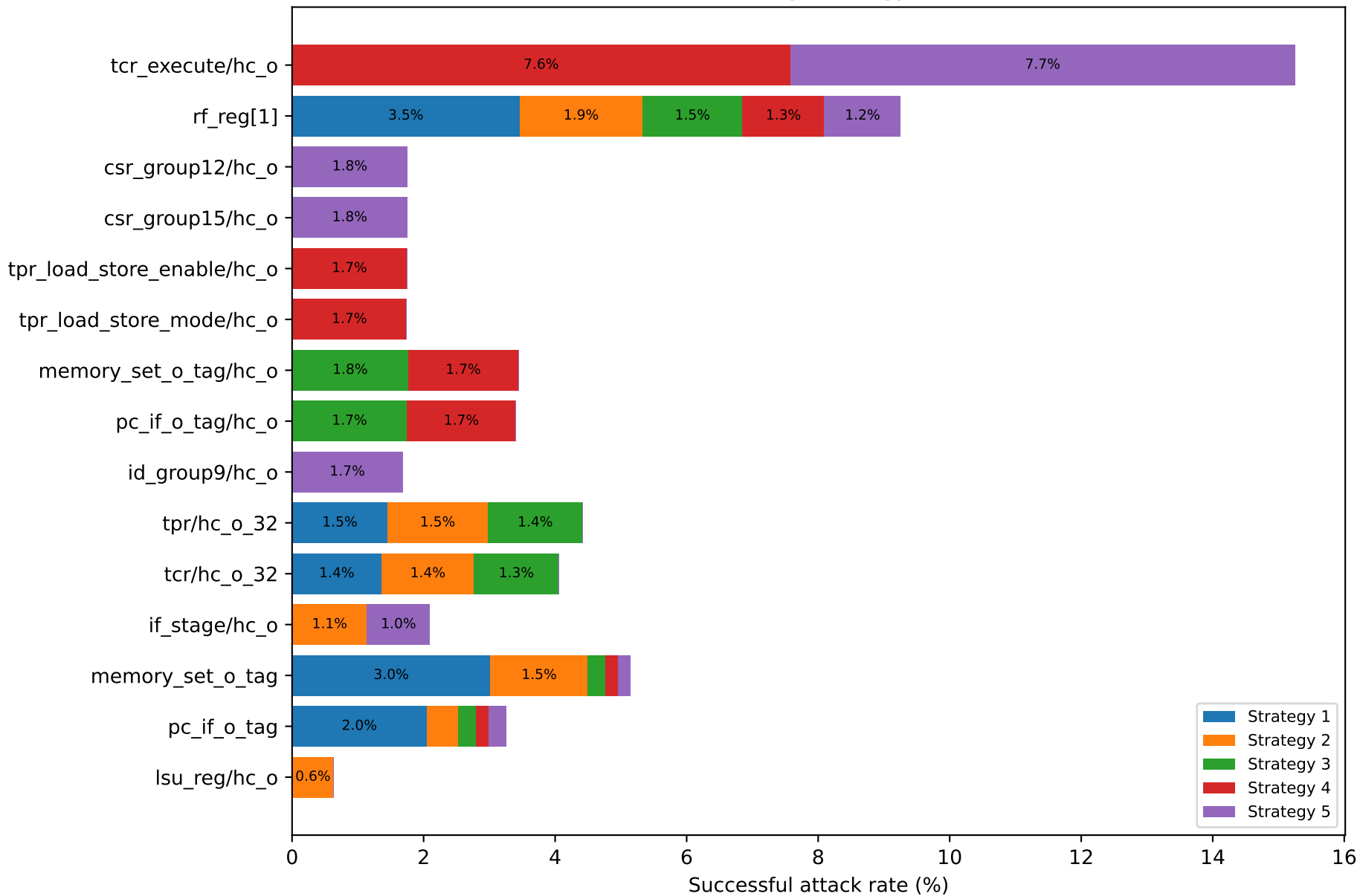
Successful attack rate by strategy — Buffer Overflow
