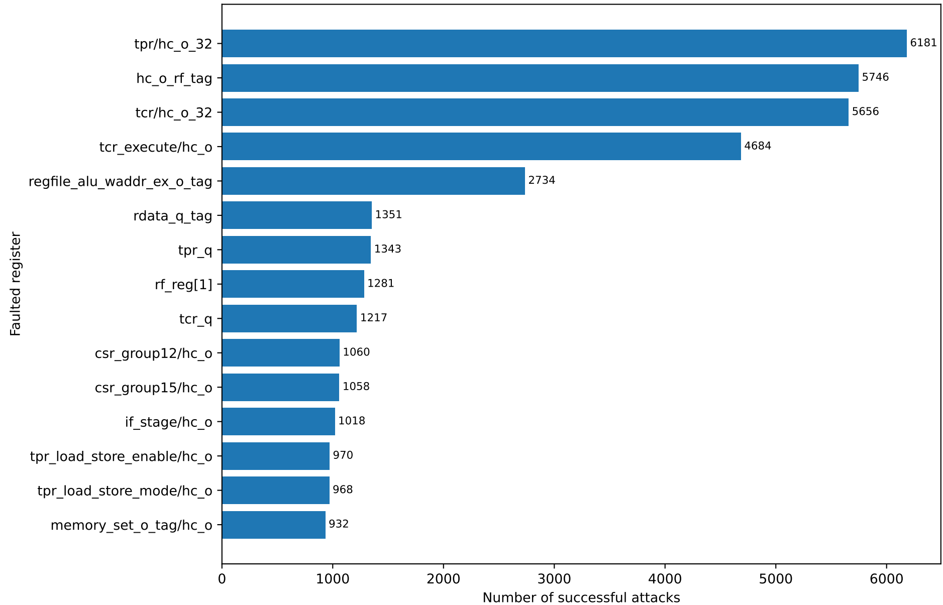
Registers with the highest number of successful attacks — Buffer Overflow
