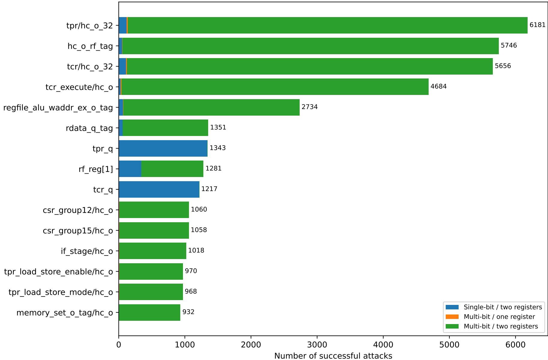
Successful attacks by fault model — Buffer Overflow
