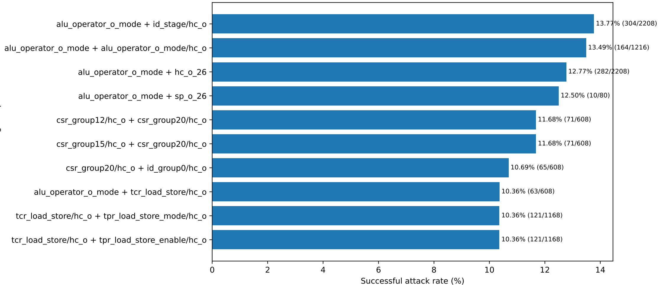
Most vulnerable register pairs — Format String
