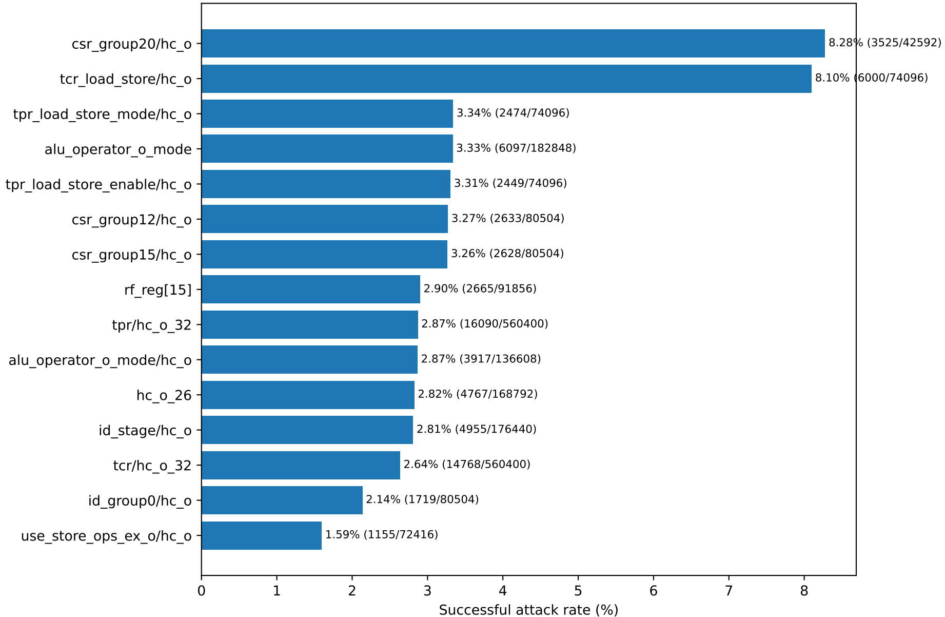
Most vulnerable registers — Format String
