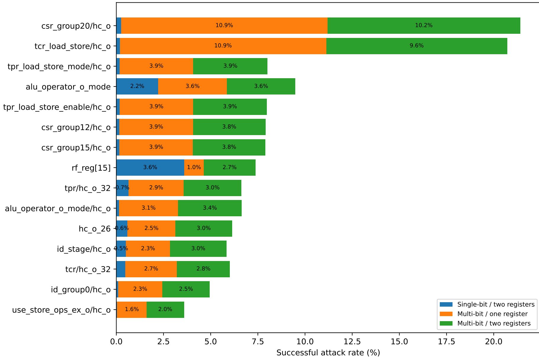
Successful attack rate by fault model — Format String
