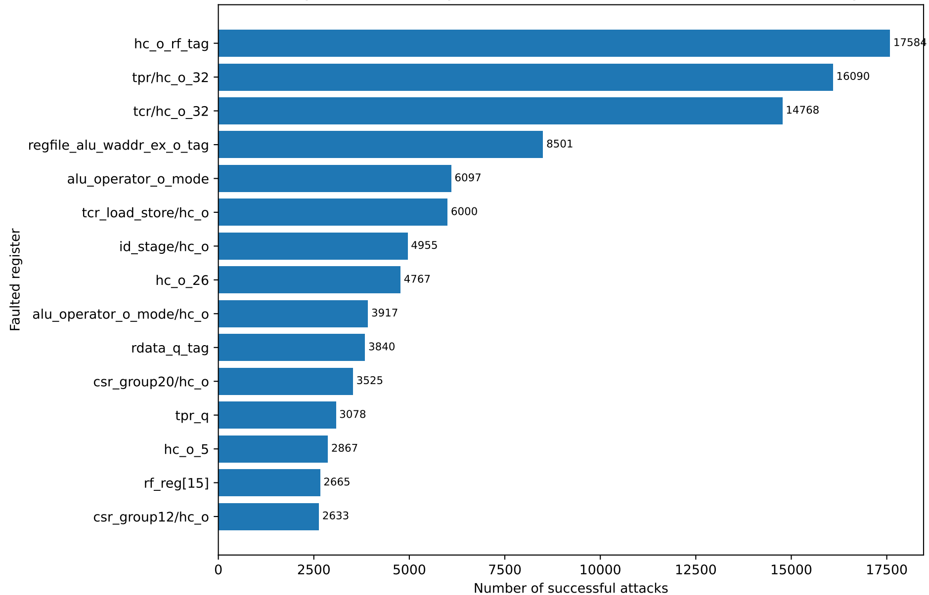
Registers with the highest number of successful attacks — Format String
