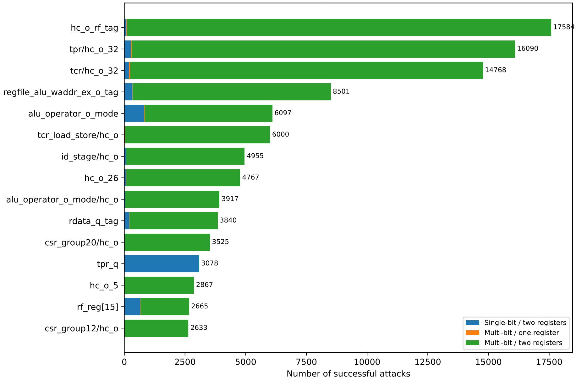
Successful attacks by fault model — Format String
