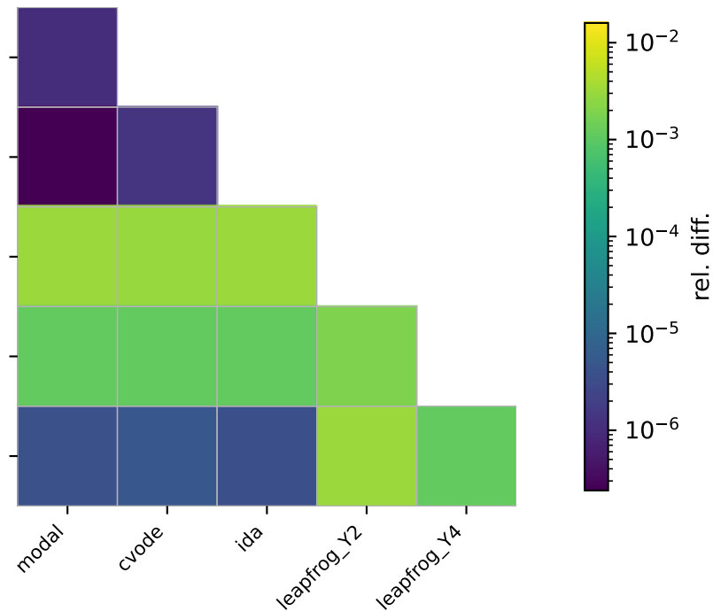
Coupled-scalar two-channel mixing
