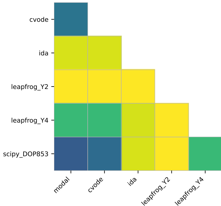
Einstein-Maxwell Gertsenshtein
