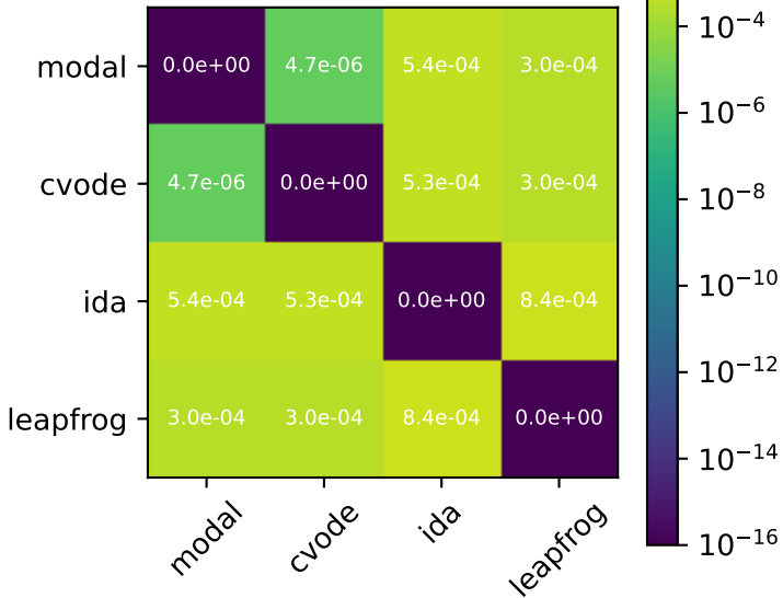
gertsenshtein
