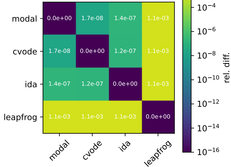
coupled_scalars
