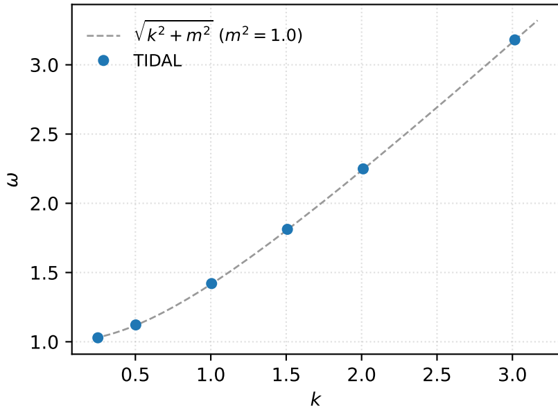
(a) Proca dispersion
