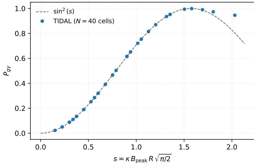
(b) universal-collapse plot
