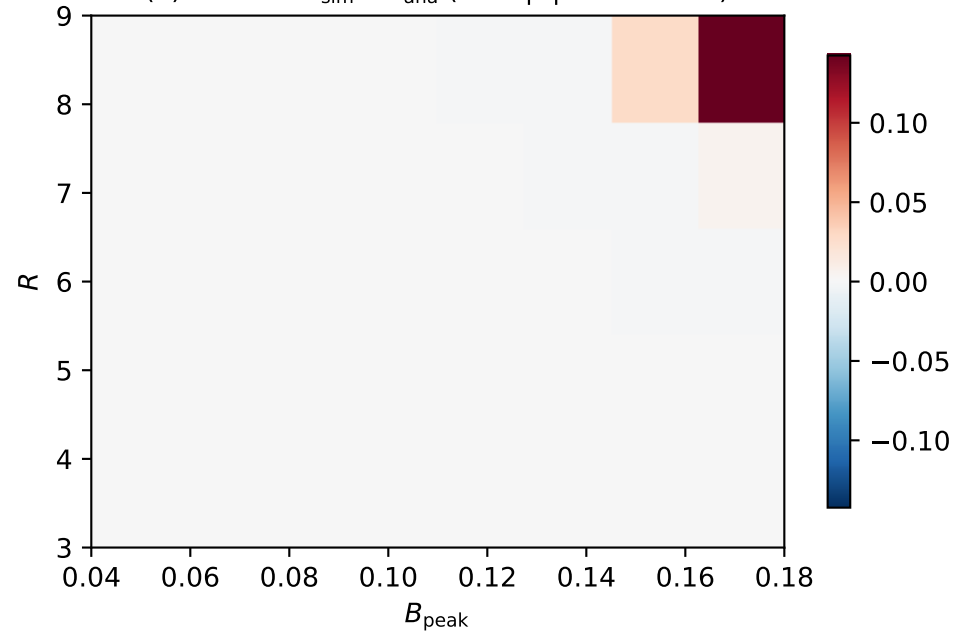
(a) residual P_{\text{sim}} - P_{\text{ana}} ( \max |\Delta| = 1.4e - 01 )
