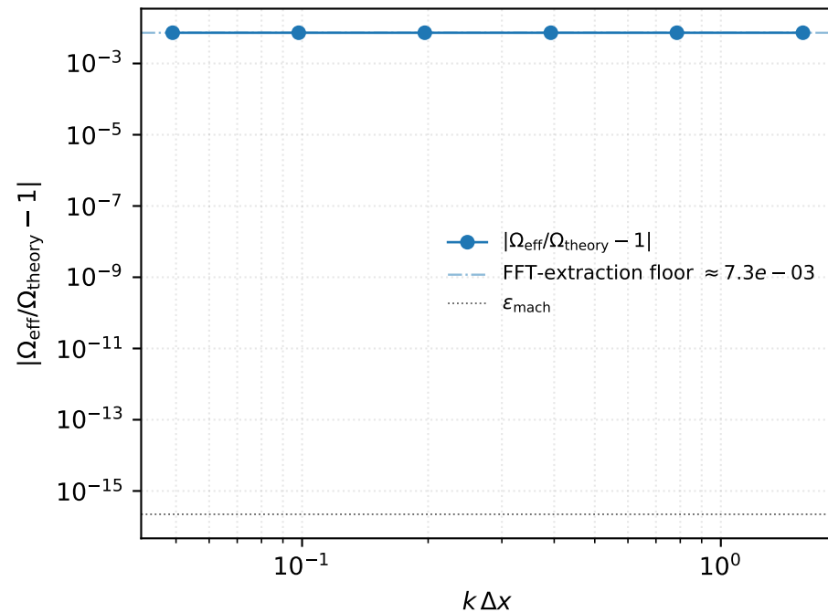
(b) Rabi-frequency grid convergence
