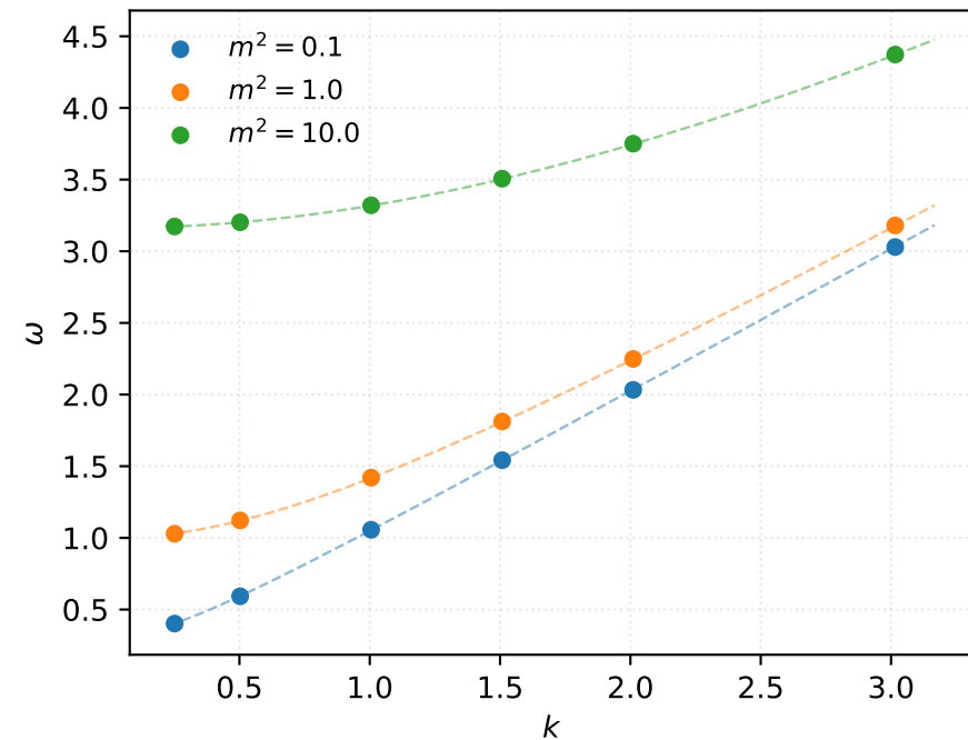
(a) Proca dispersion
