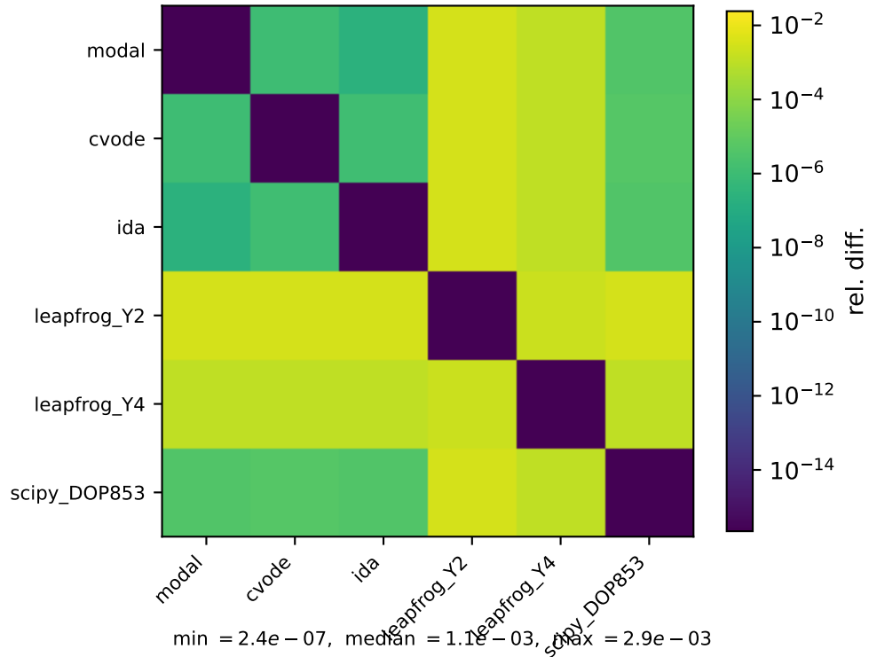
Coupled-scalar two-channel mixing
