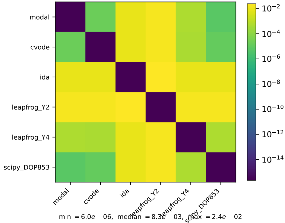
Einstein-Maxwell Gertsenshtein
