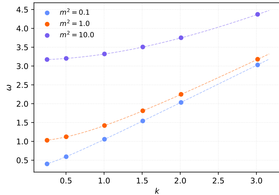
(a) Proca dispersion
