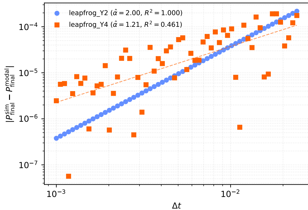
(b) time-integration order (leapfrog only)
