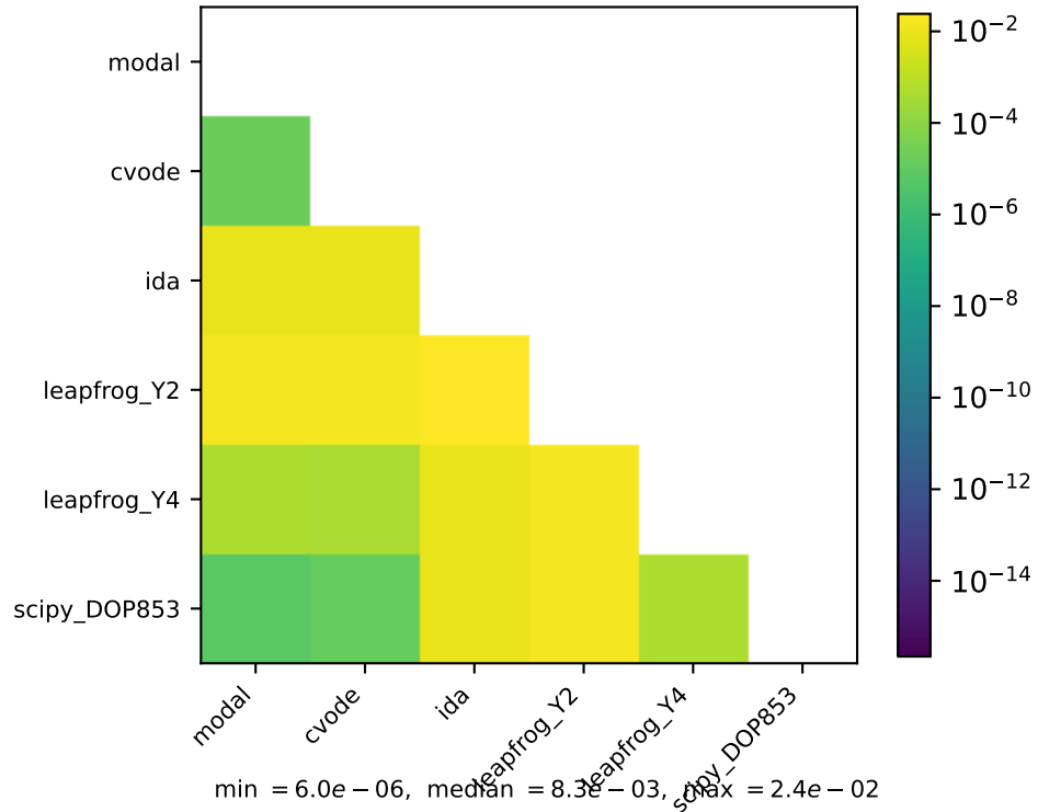
Einstein-Maxwell Gertsenshtein
