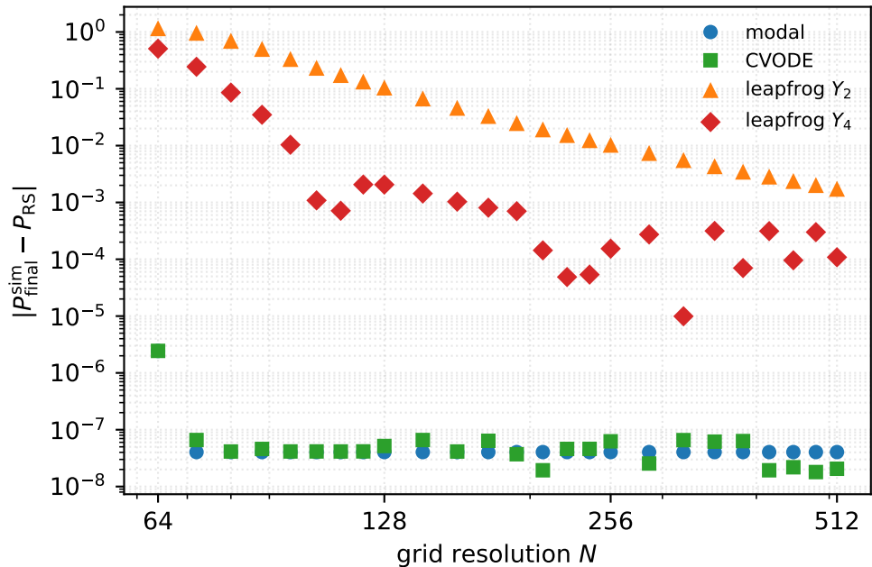
(b) N -convergence at B_0 = 0.1275
