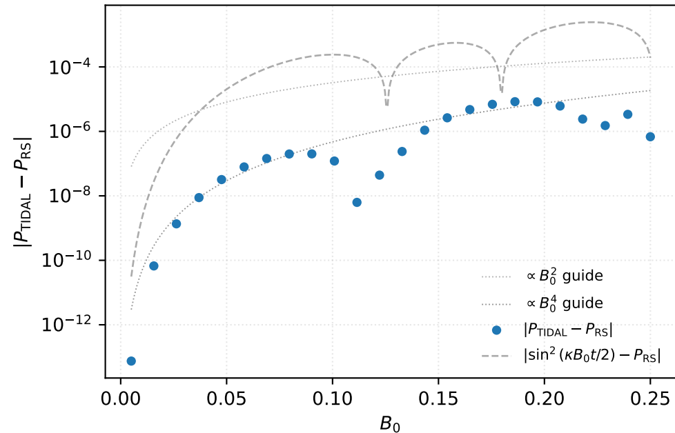
(a) residual at t = 50
