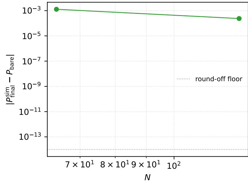
(c) N-convergence
