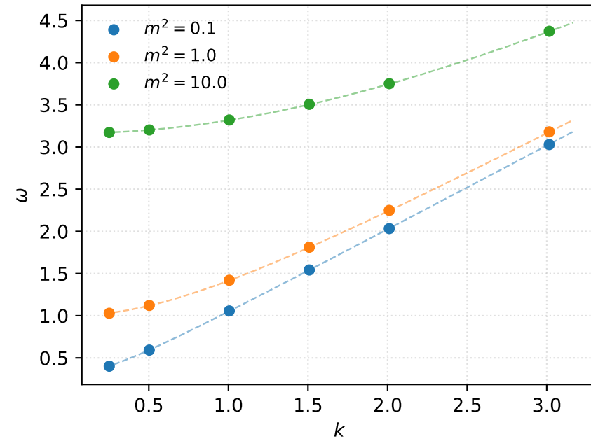
(a) Proca dispersion
