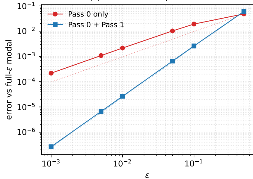
(a) error vs \varepsilon — slope \approx 1.99
