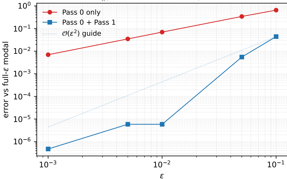
\varepsilon \cdot \partial_x^4 \phi correction — fitted slope \approx 2.59
