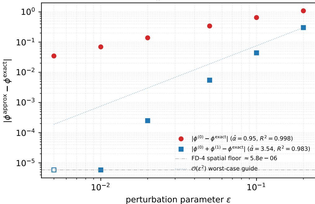
\varepsilon \partial_x^4 \phi correction
