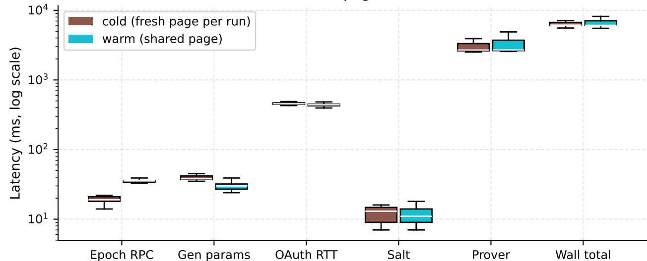
Cold (n=30) vs warm (n=30) page context, N=3 cache=none
