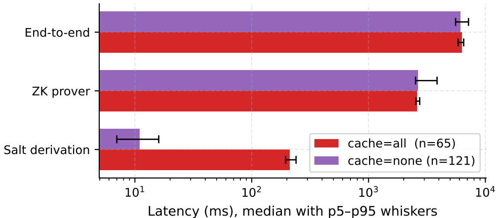
Cache ablation at N=3 (whiskers span p5-p95)
