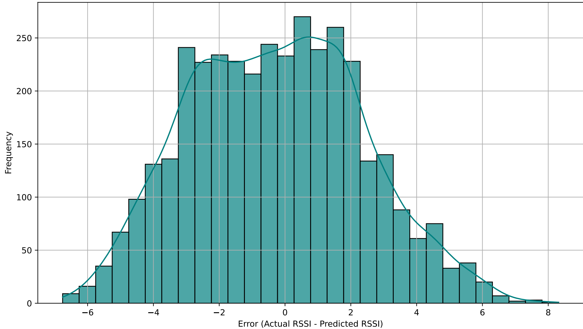
Distribution of Prediction Errors (Last Step - step 75 \approx 3.0 s)
