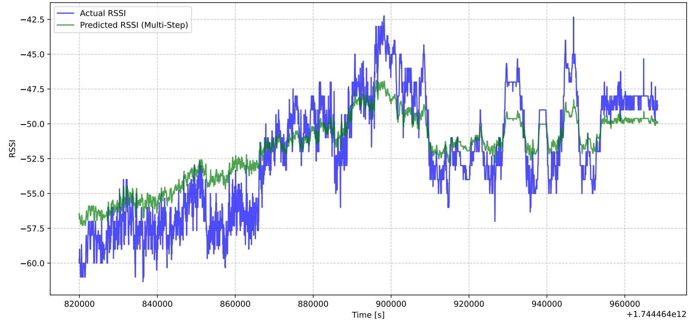
Actual vs Predicted RSSI (Multi-Step (step 75 \approx 3.0 s))
