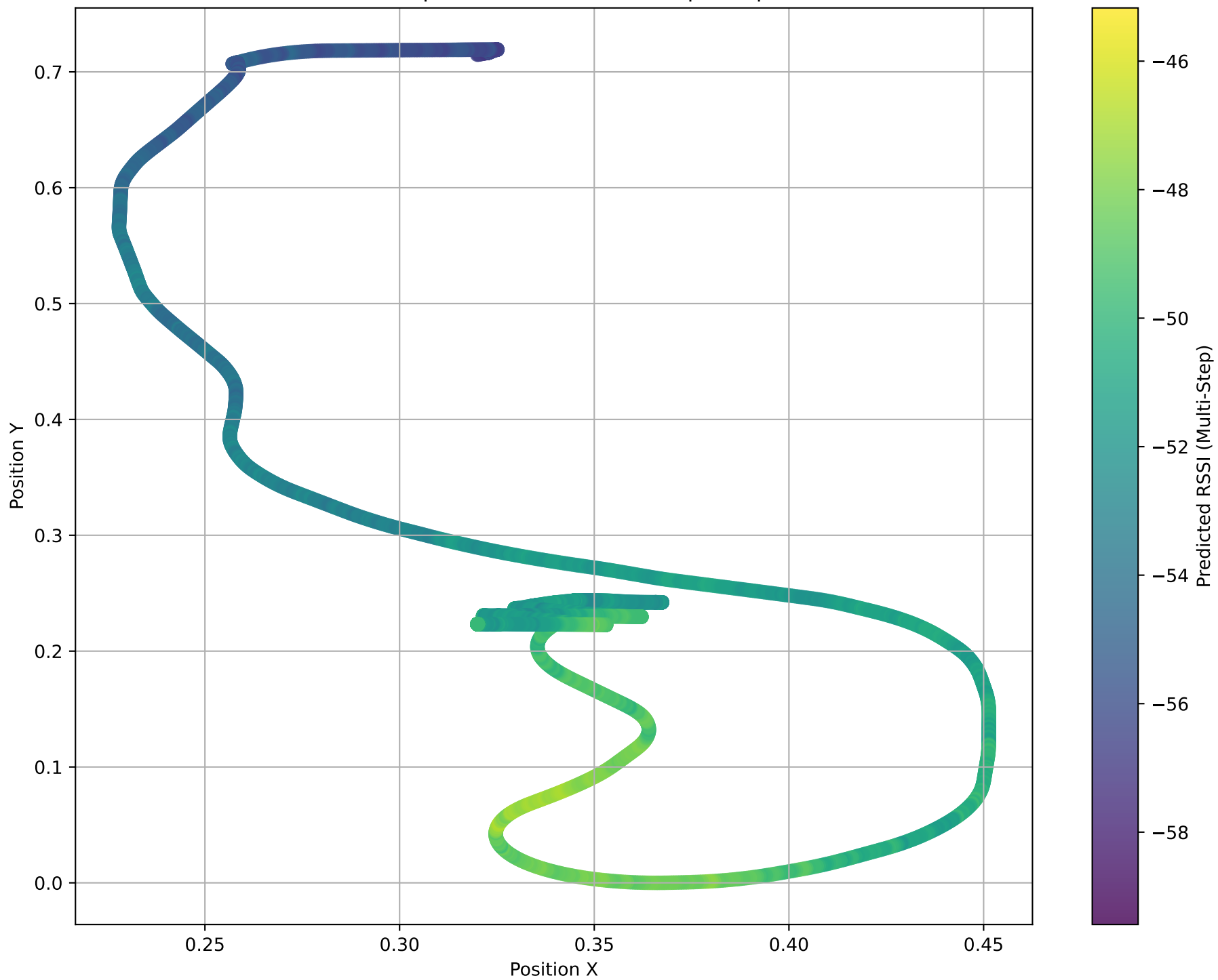
Predicted RSSI in Spatial Context (Multi-Step - step 75 \approx 3.0 s)
