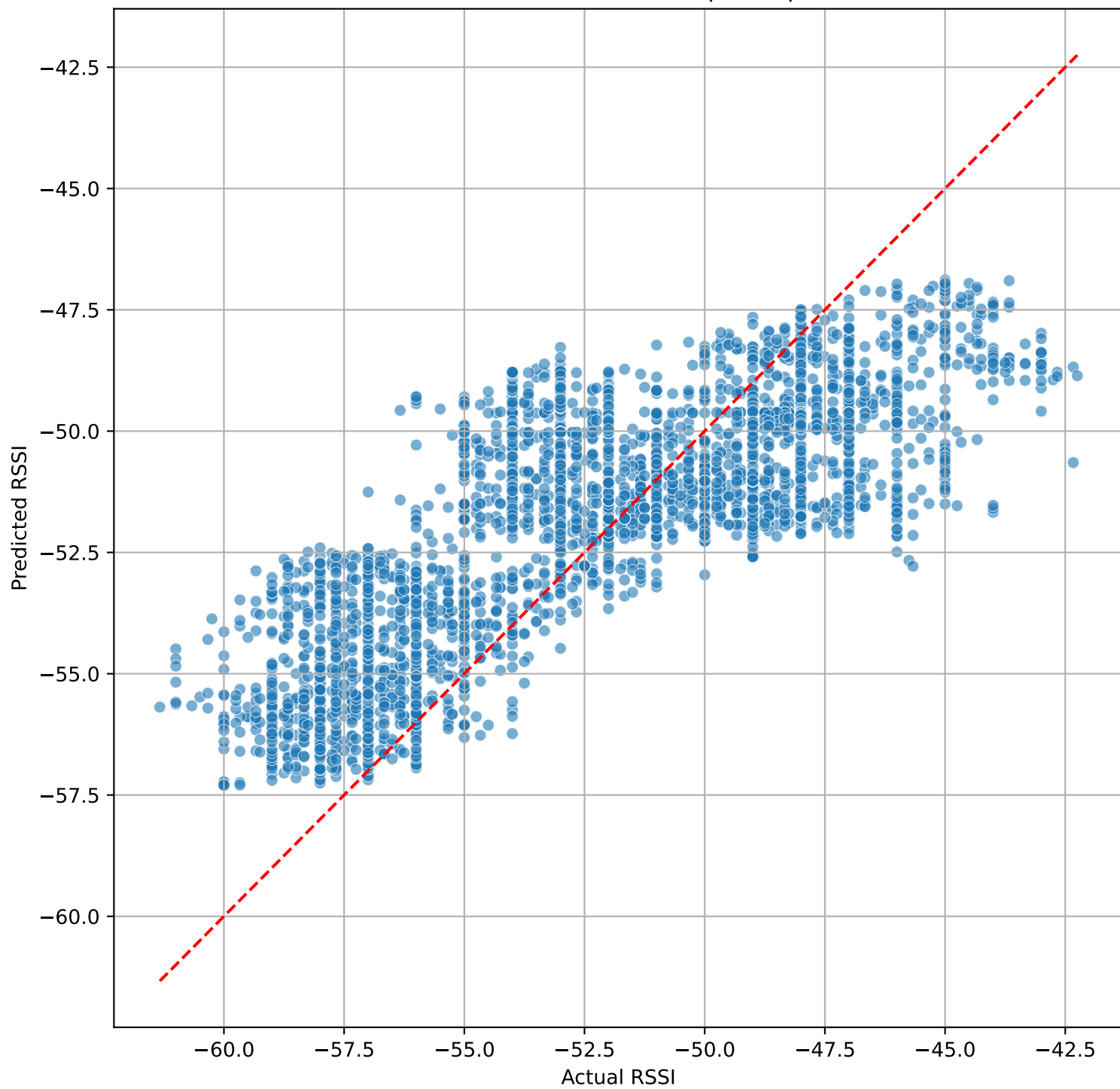
Actual vs Predicted RSSI (Last Step - step 75 \approx 3.0 s)
