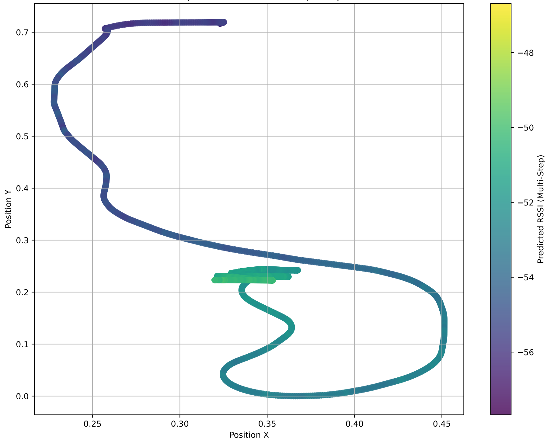
Predicted RSSI in Spatial Context (Multi-Step - step 200 \approx 8.0 s)
