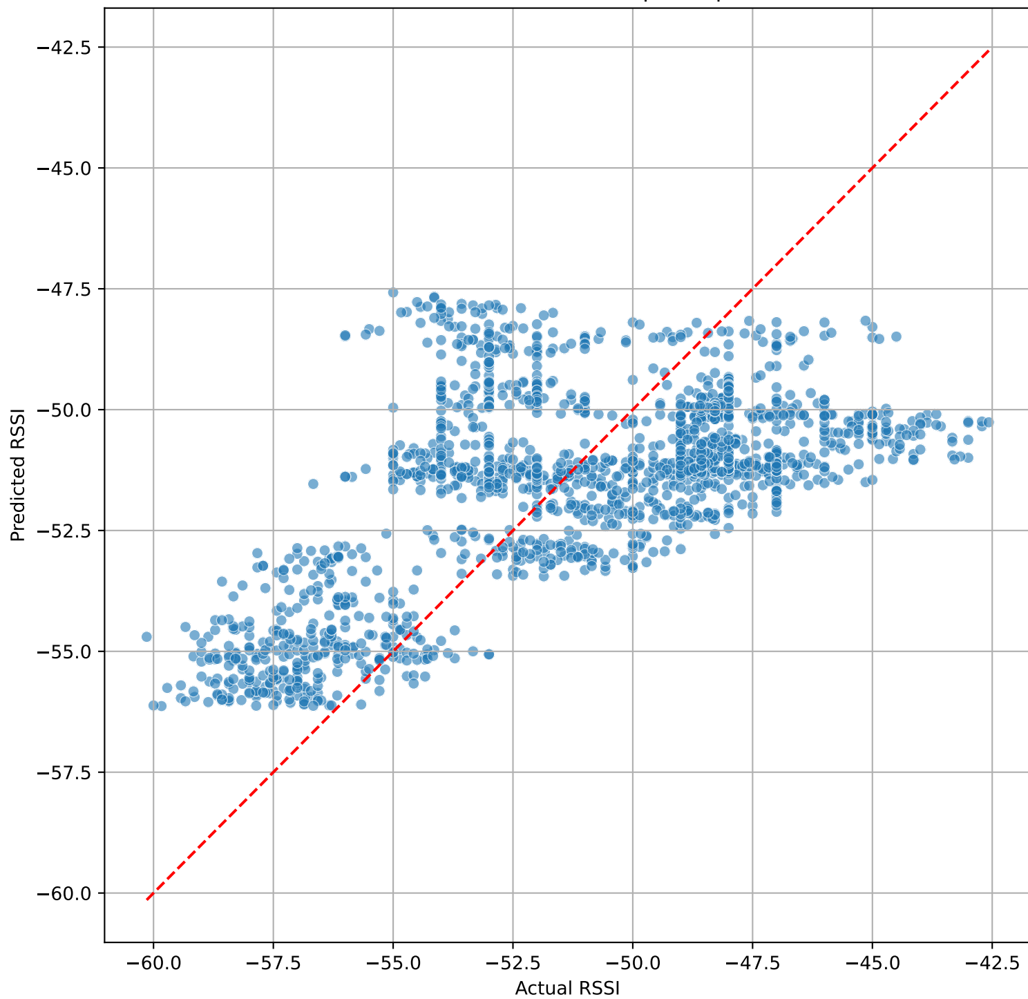
Actual vs Predicted RSSI (Last Step - step 200 \approx 8.0 s)
