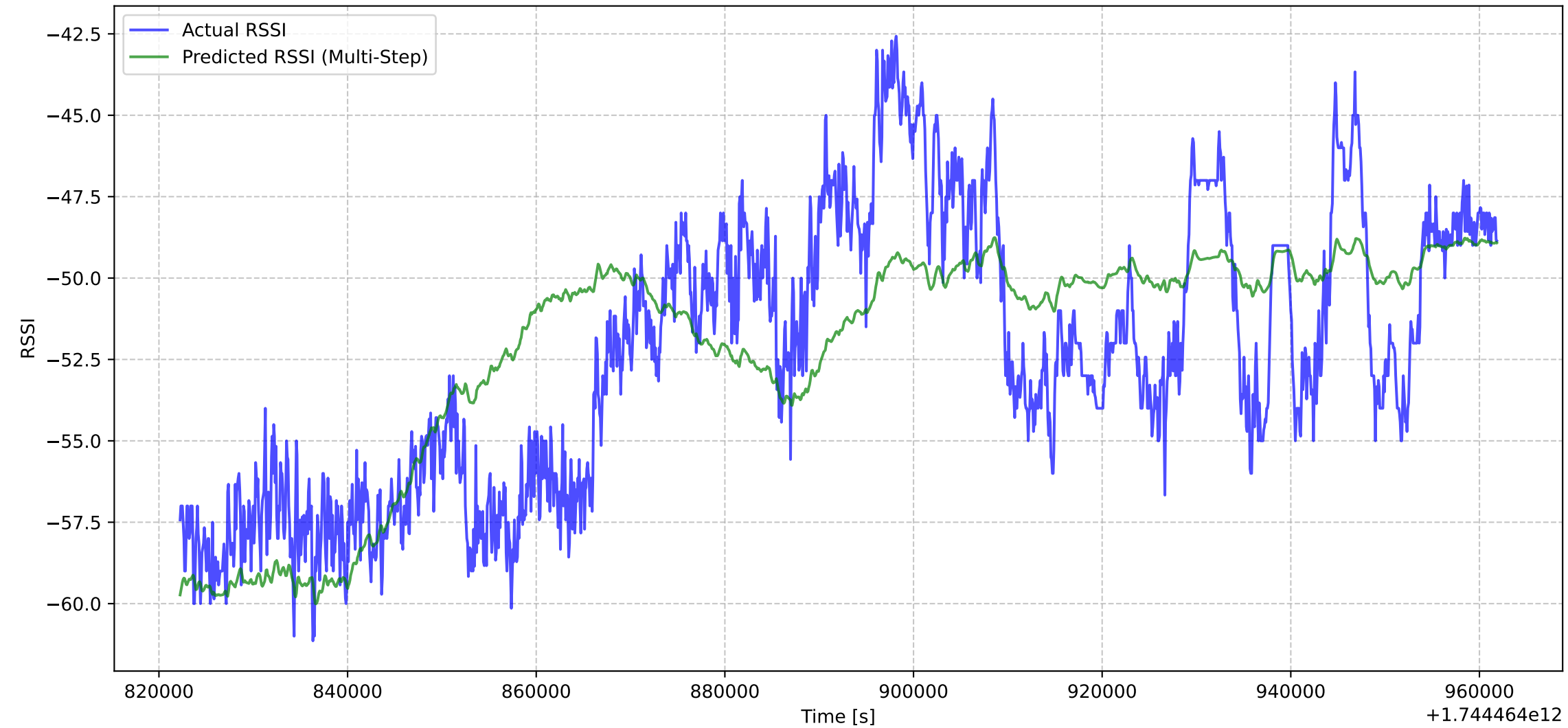
Actual vs Predicted RSSI (Multi-Step (step 120 \approx 10.0 s))
