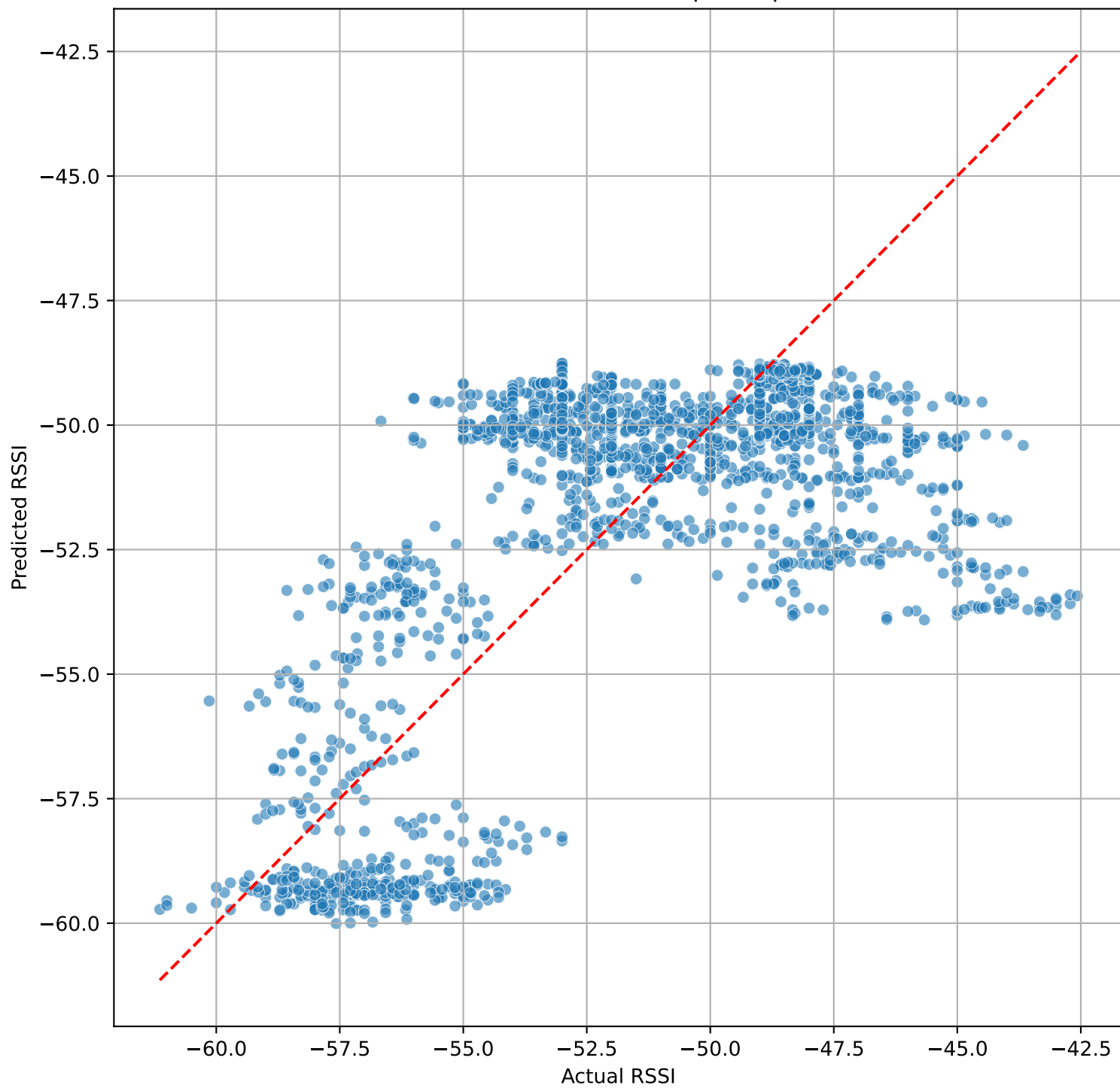
Actual vs Predicted RSSI (Last Step - step 120 \approx 10.0 s)
