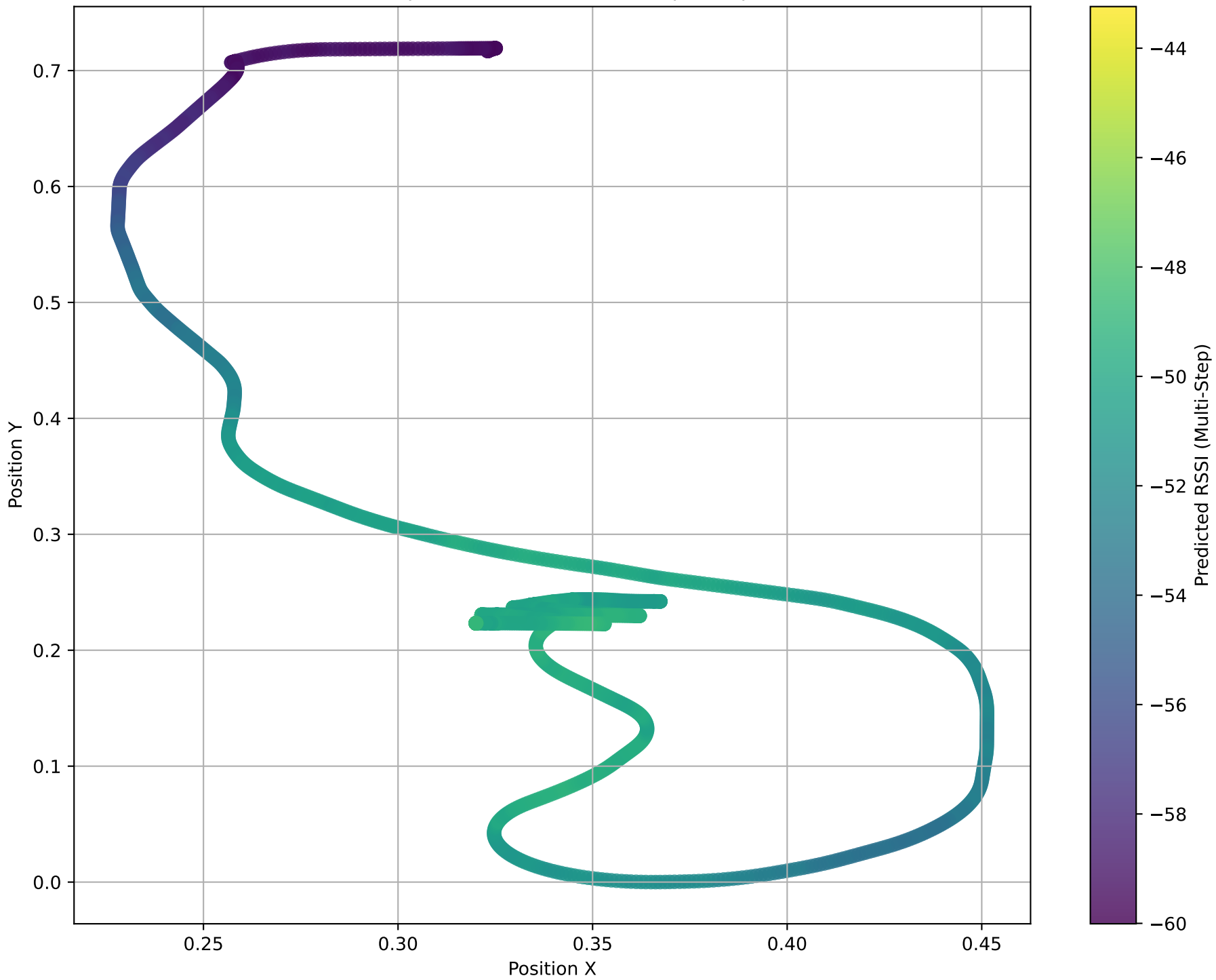
Predicted RSSI in Spatial Context (Multi-Step - step 120 \approx 10.0 s)
