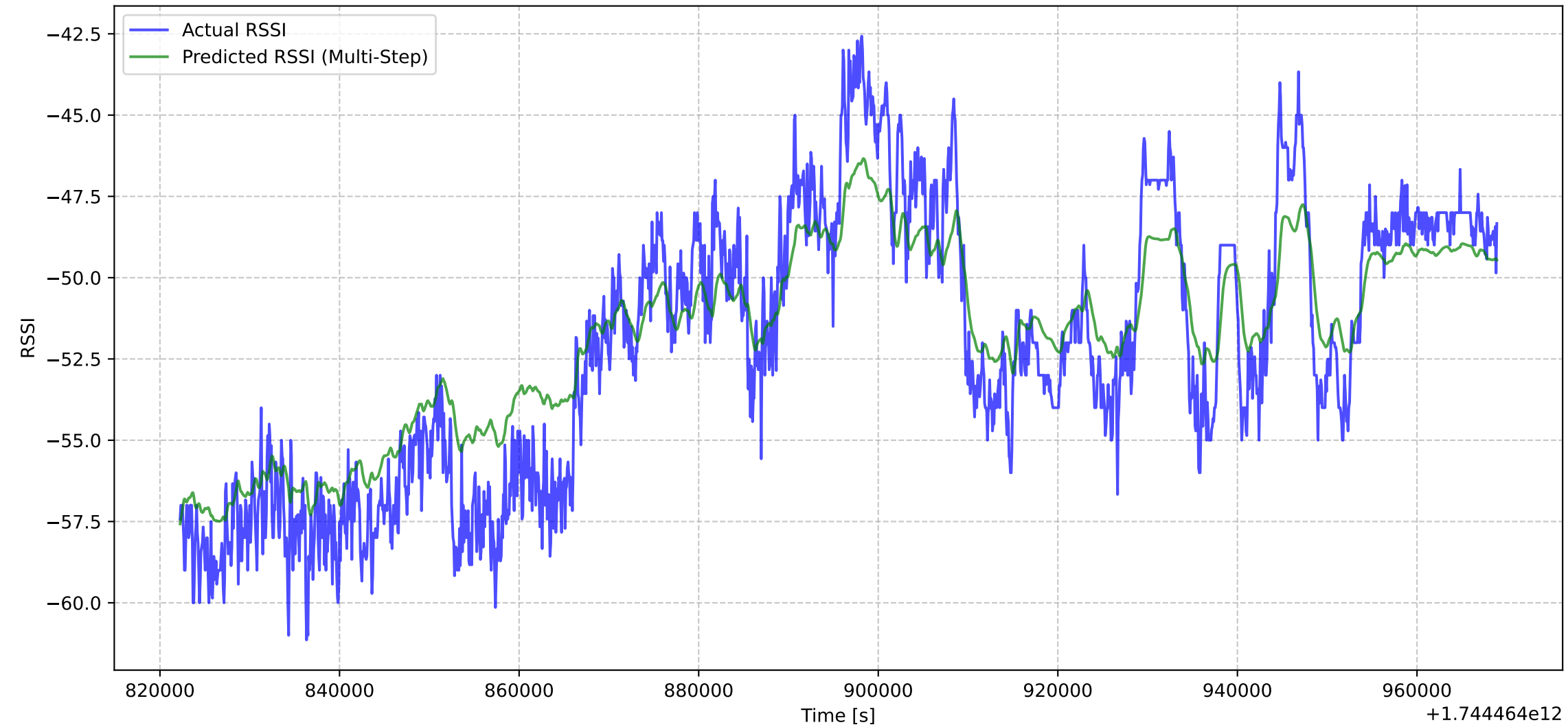
Actual vs Predicted RSSI (Multi-Step (step 32 \approx 4.0 s))
