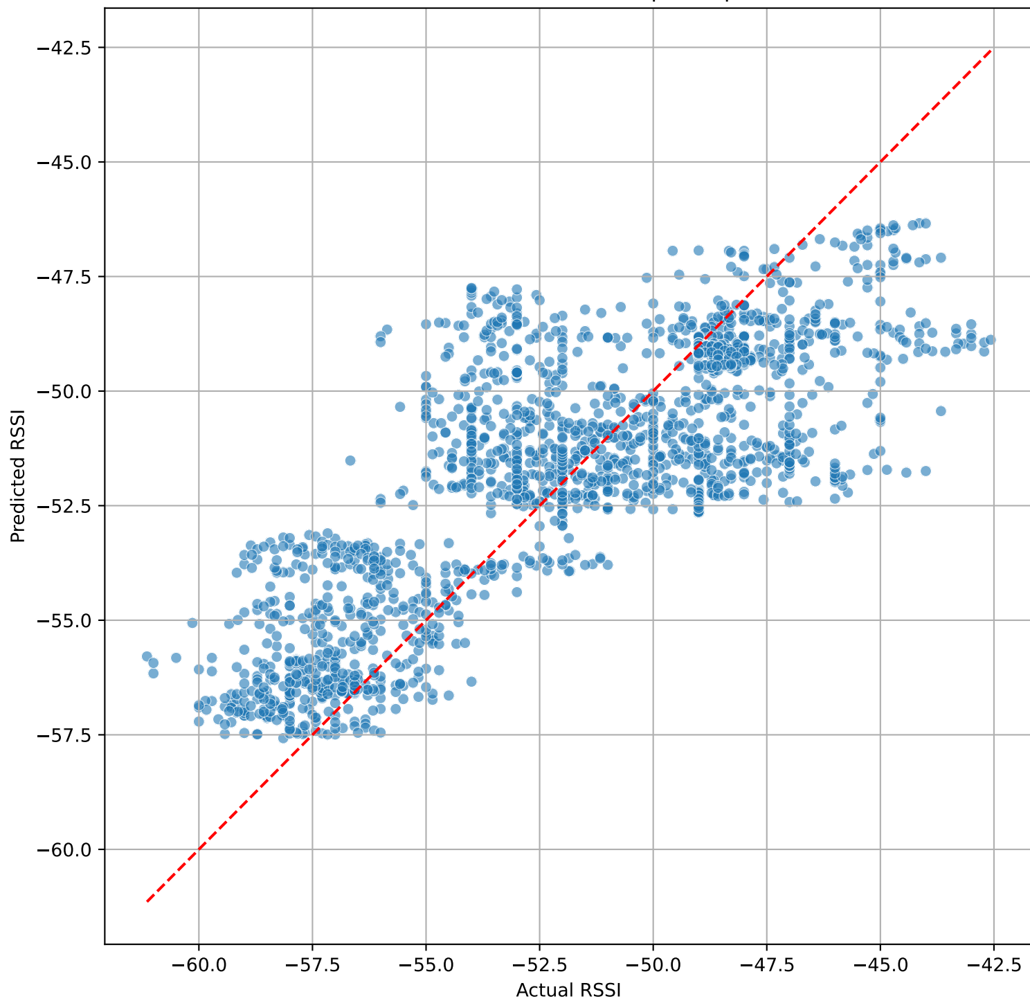
Actual vs Predicted RSSI (Last Step - step 32 \approx 4.0 s)
