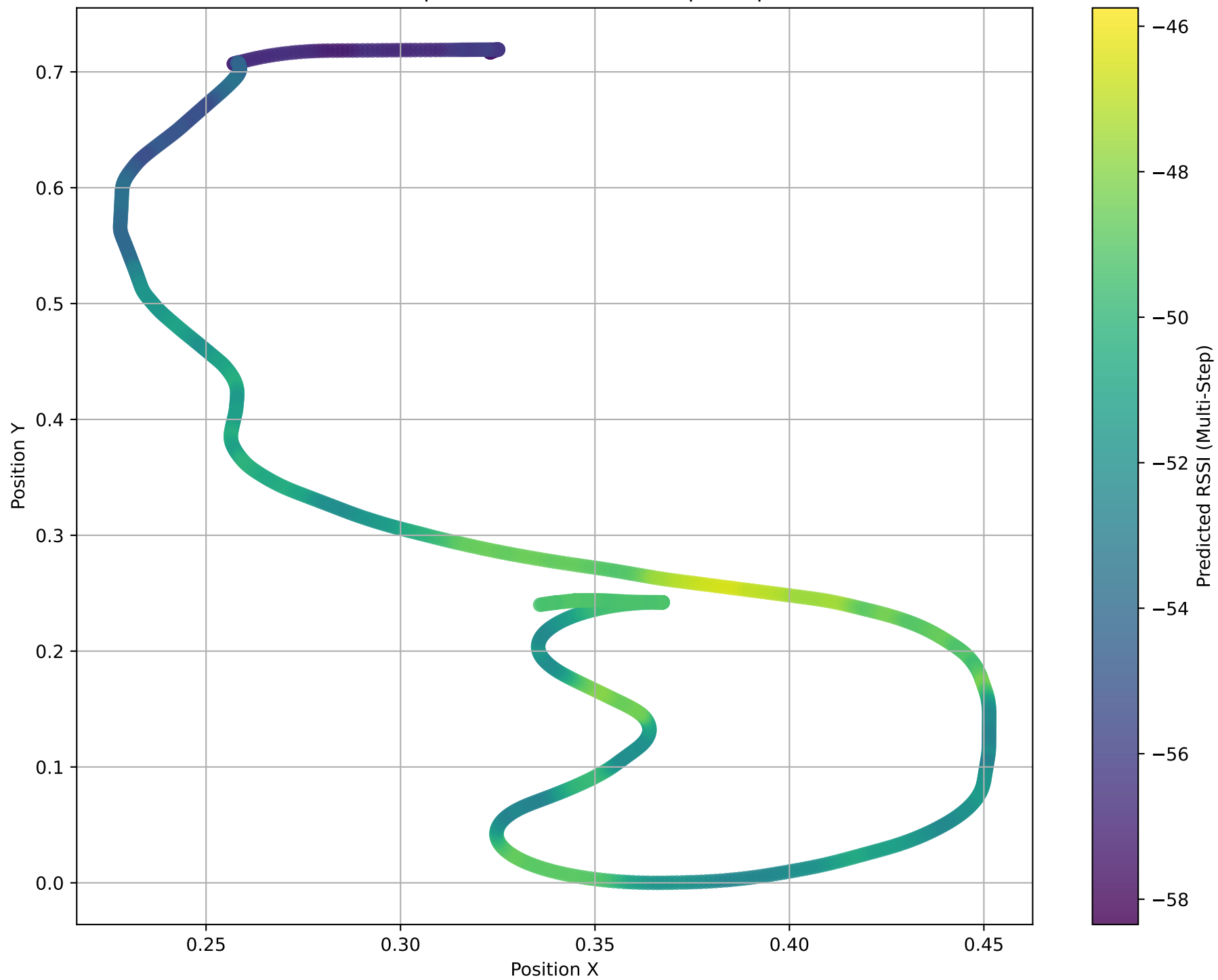
Predicted RSSI in Spatial Context (Multi-Step - step 32 \approx 4.0 s)
