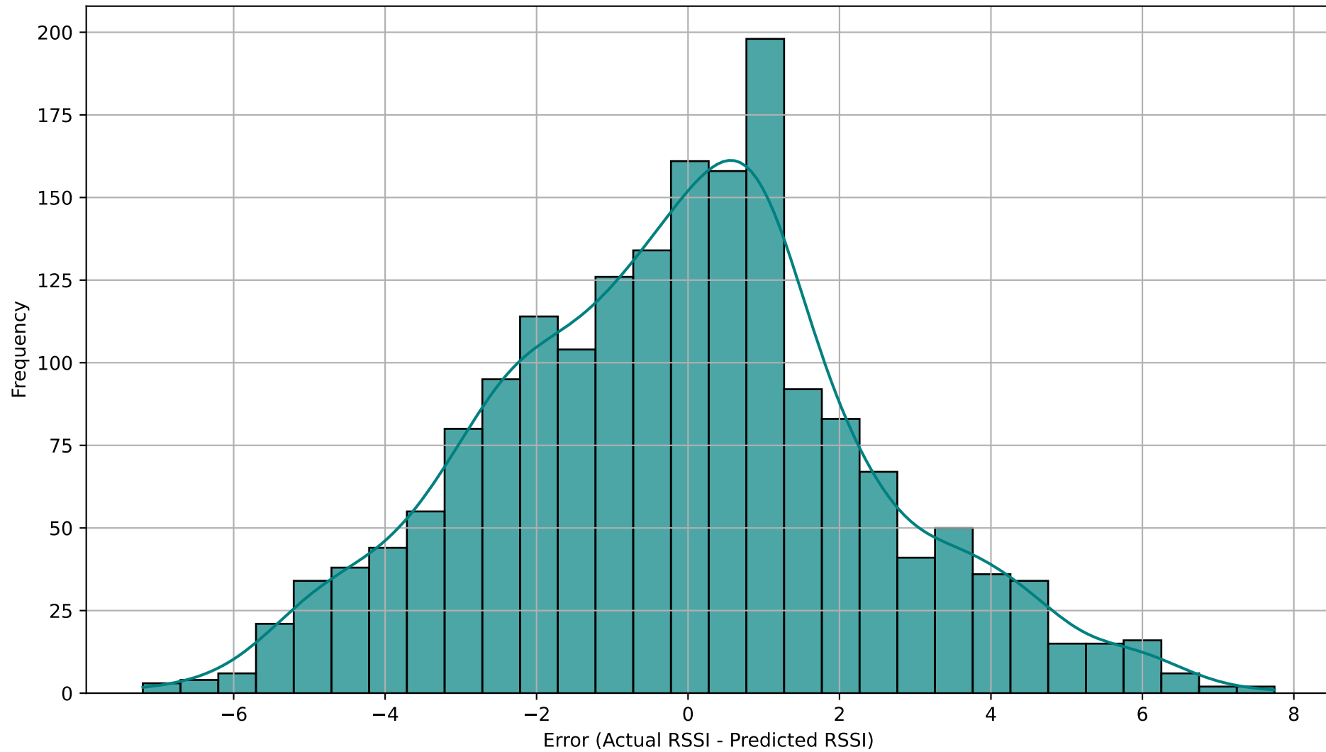
Distribution of Prediction Errors (Last Step - step 32 \approx 4.0 s)
