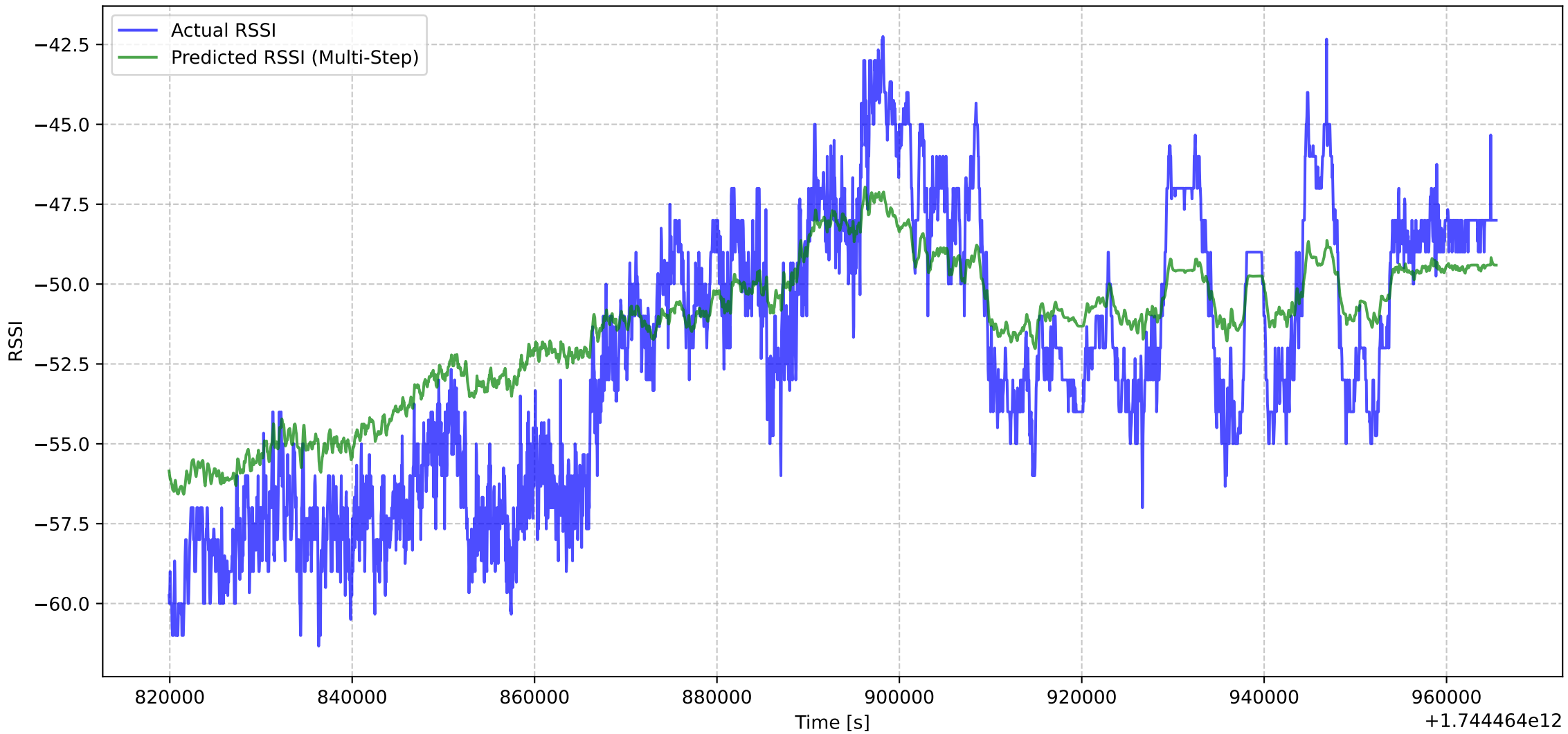
Actual vs Predicted RSSI (Multi-Step (step 150 \approx 6.0 s))
