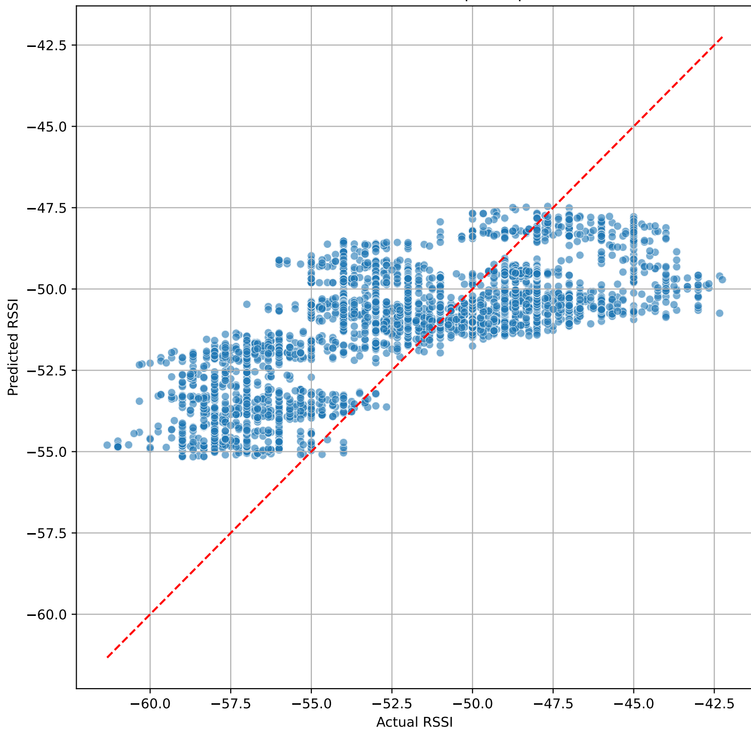
Actual vs Predicted RSSI (Last Step - step 250 \approx 10.0 s)
