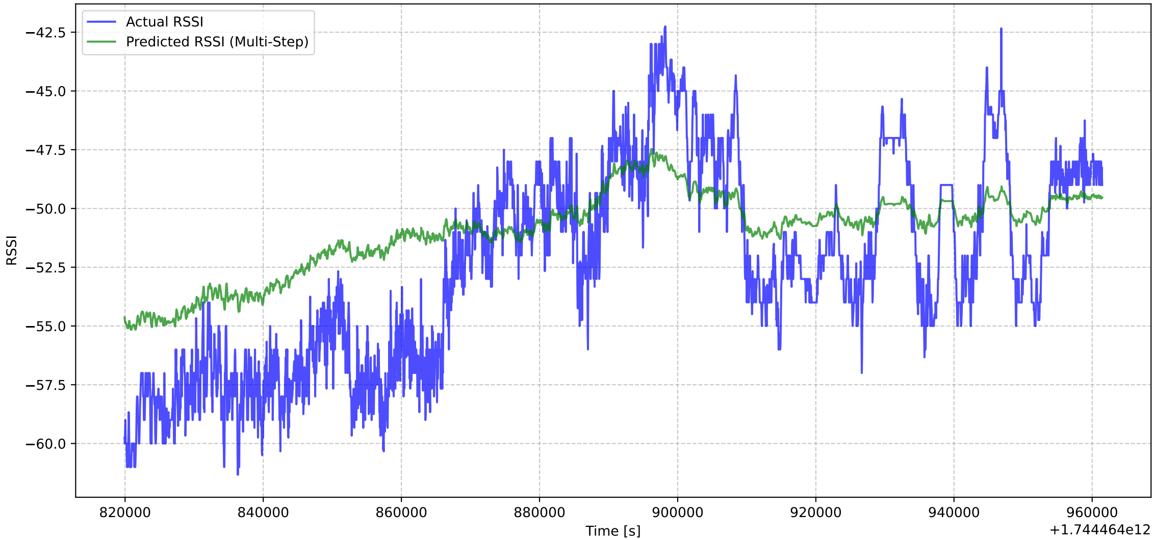
Actual vs Predicted RSSI (Multi-Step (step 250 \approx 10.0 s))
