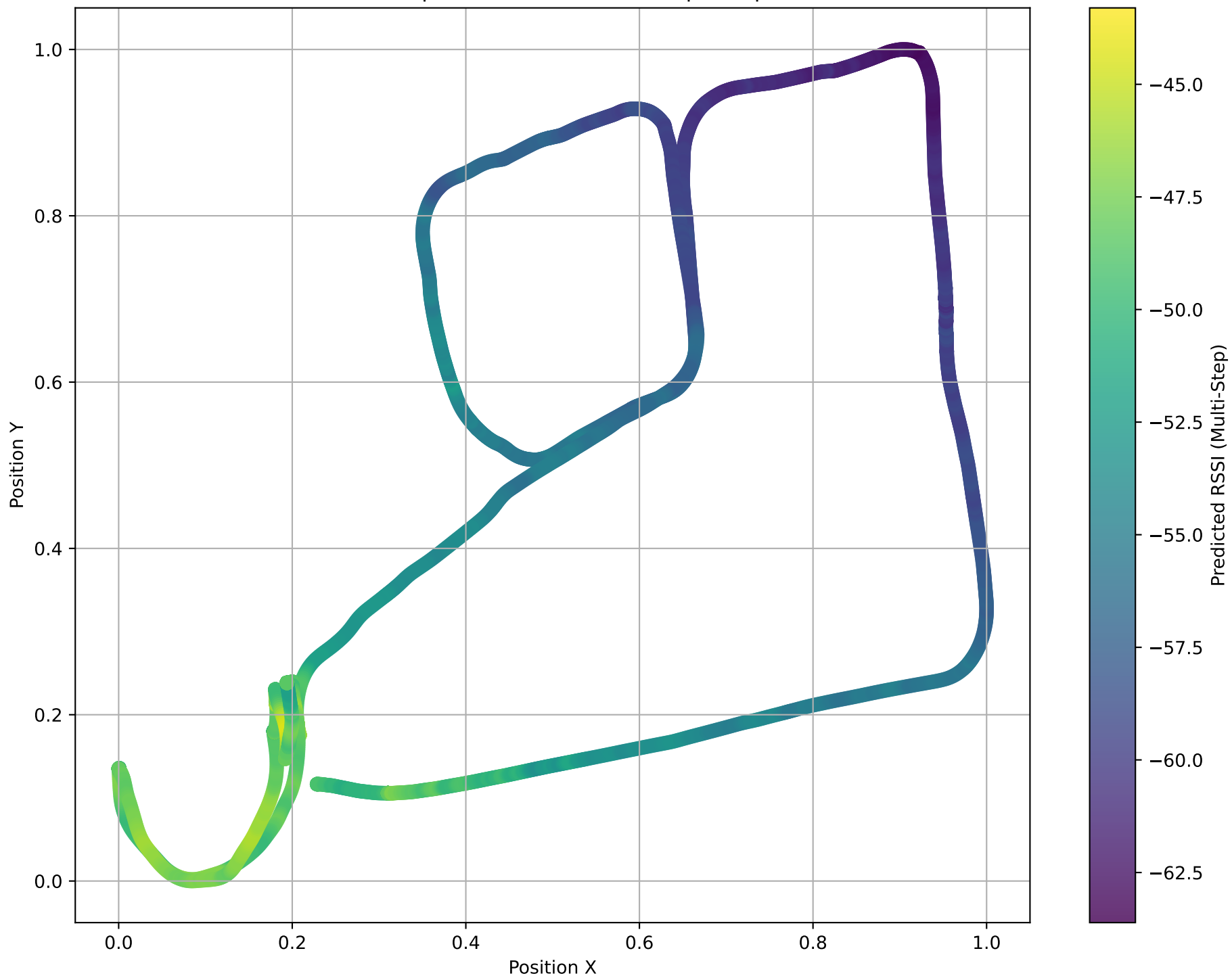
Predicted RSSI in Spatial Context (Multi-Step - step 40 \approx 4.0 s)
