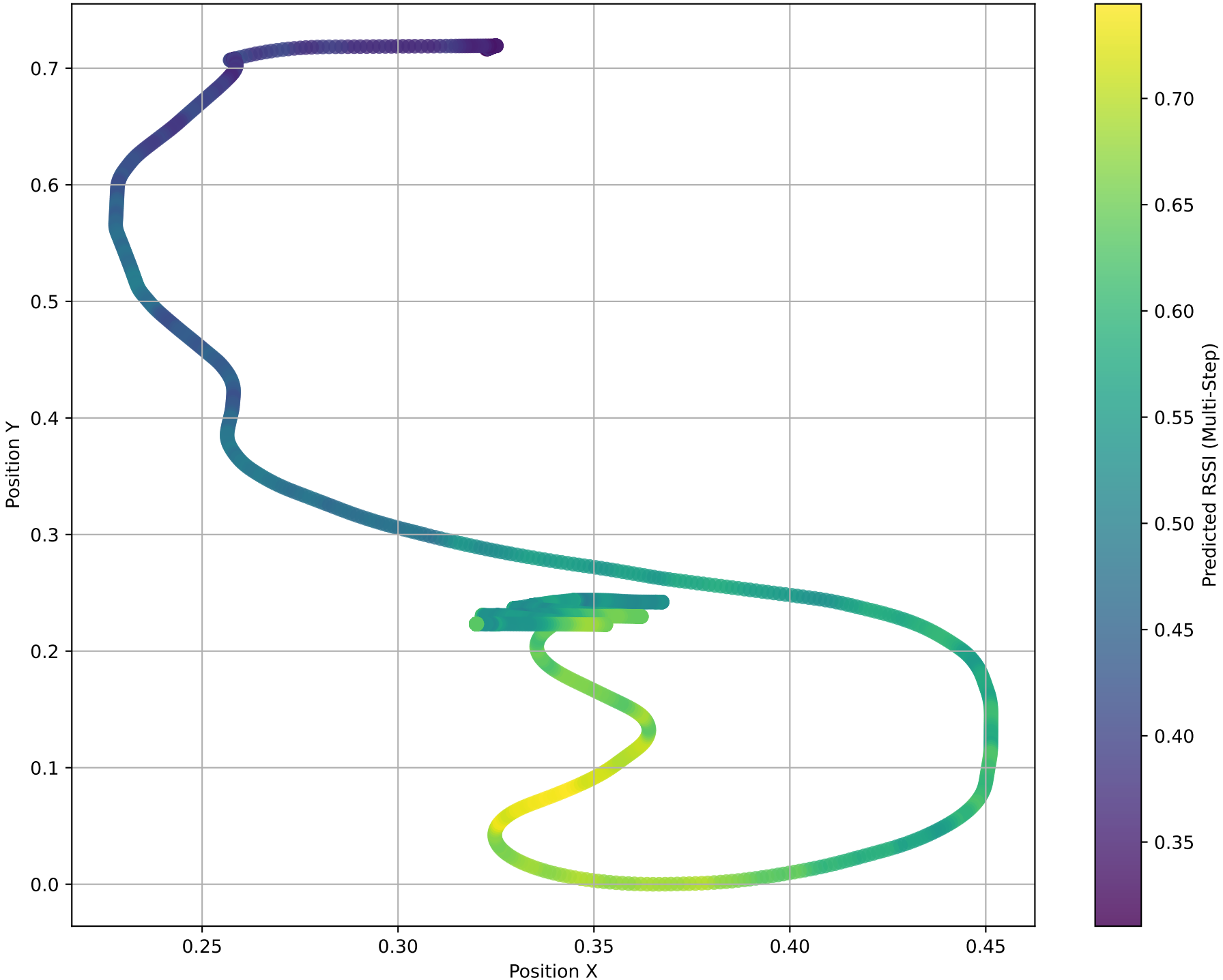
Predicted RSSI in Spatial Context (Multi-Step - step 1)
