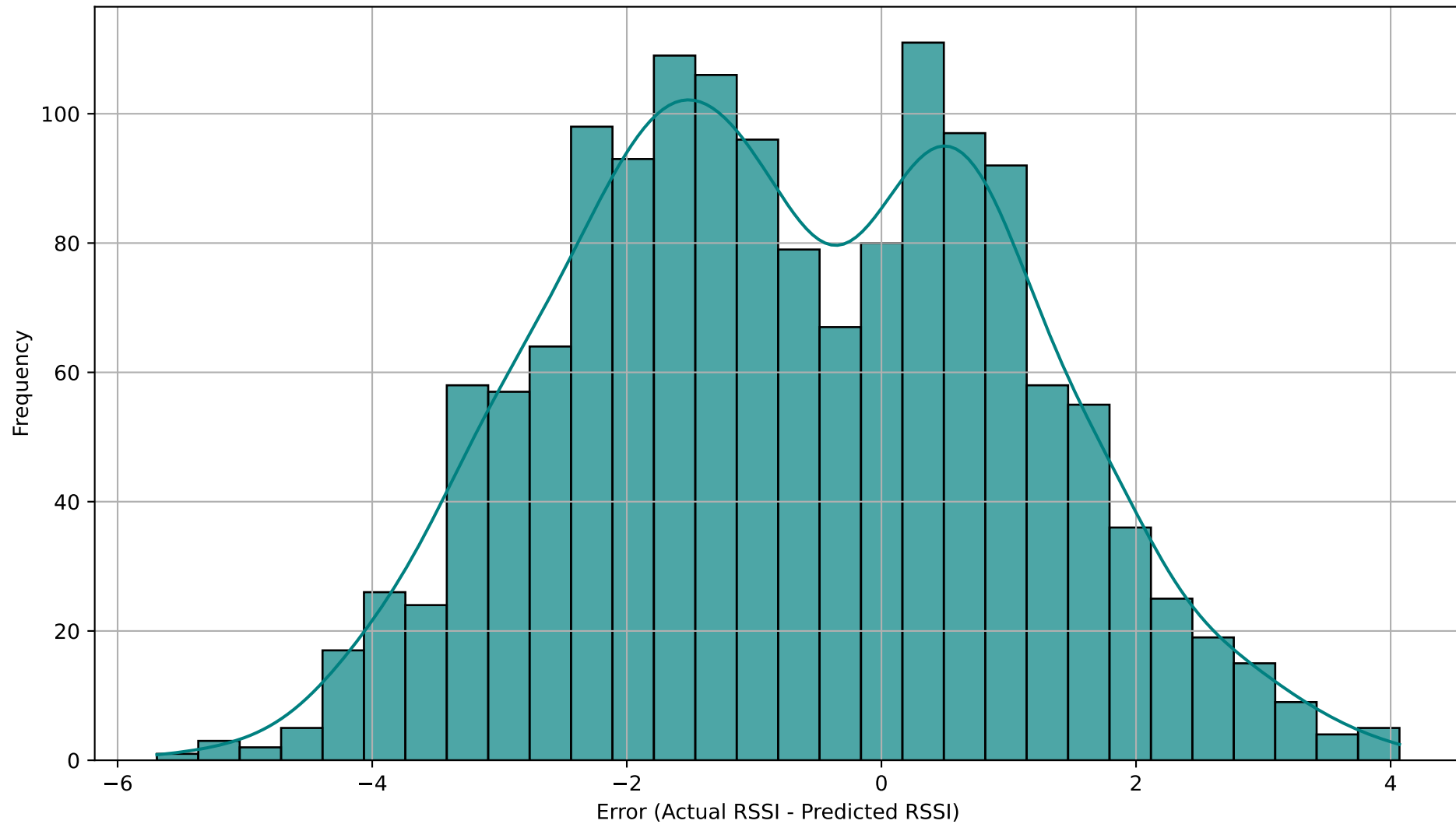
Distribution of Prediction Errors (Last Step - step 1)
