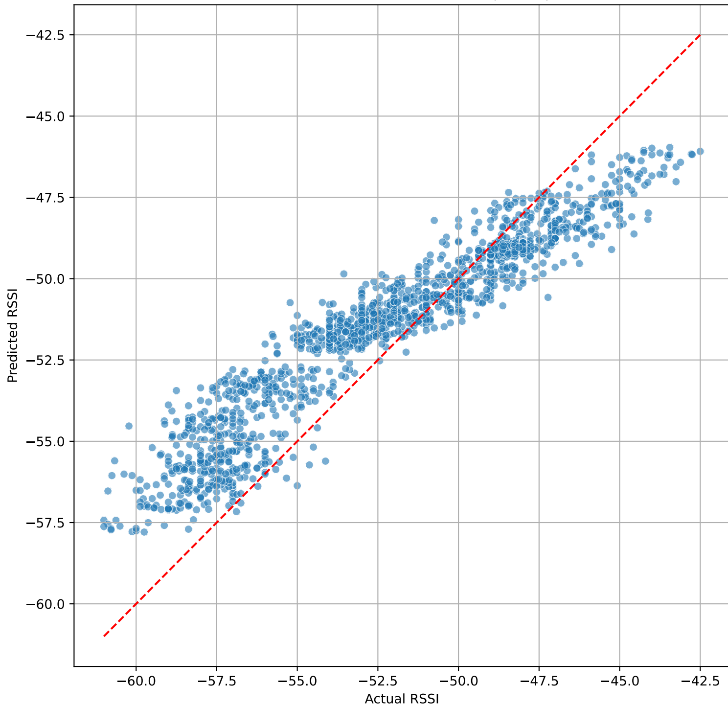
Actual vs Predicted RSSI (Last Step - step 1)
