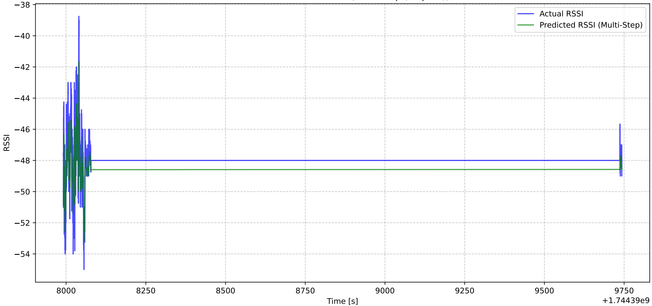
Actual vs Predicted RSSI (Multi-Step (step 40))
