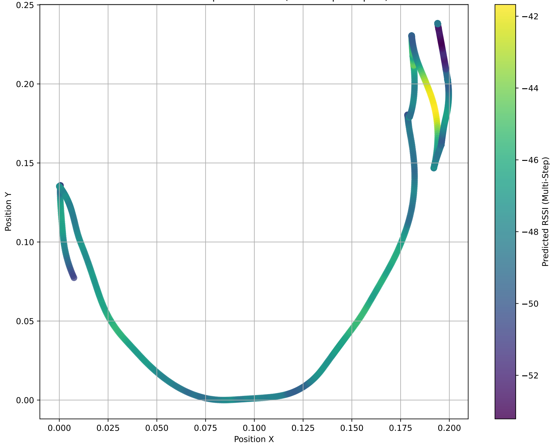
Predicted RSSI in Spatial Context (Multi-Step - step 40)
