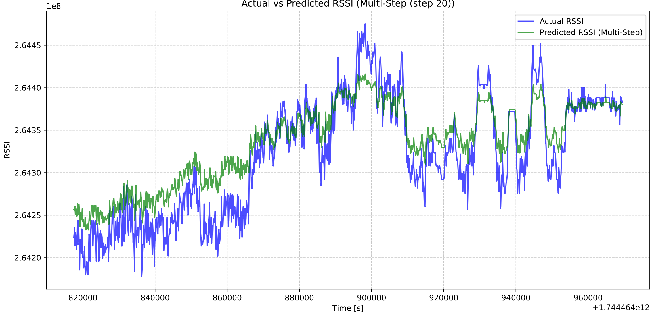
Actual vs Predicted RSSI (Multi-Step (step 20))
