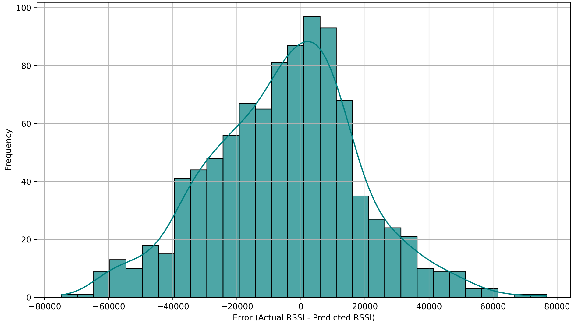
Distribution of Prediction Errors (Last Step - step 12)
