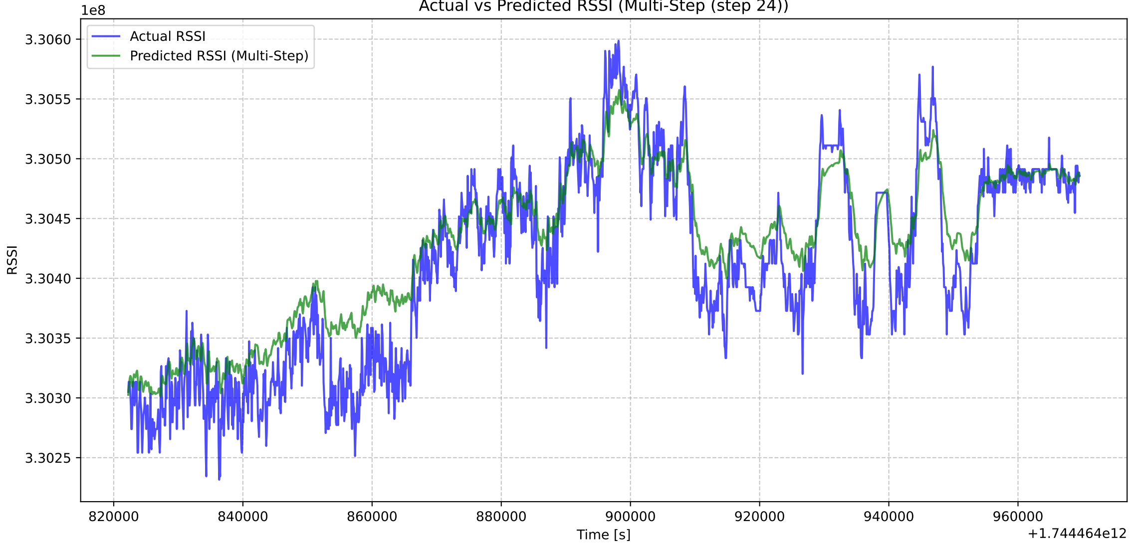
Actual vs Predicted RSSI (Multi-Step (step 24))
