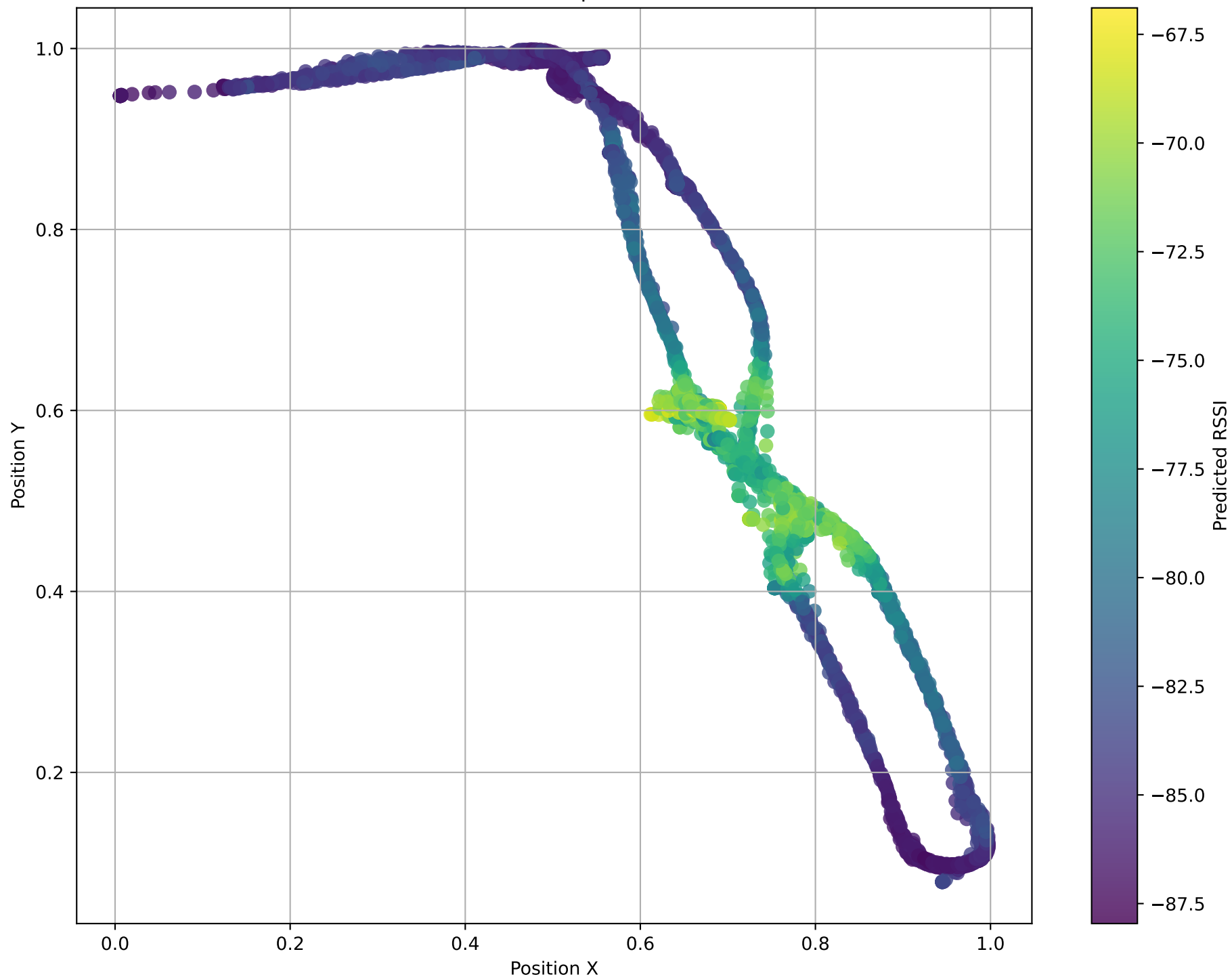
Predicted RSSI in Spatial Context
