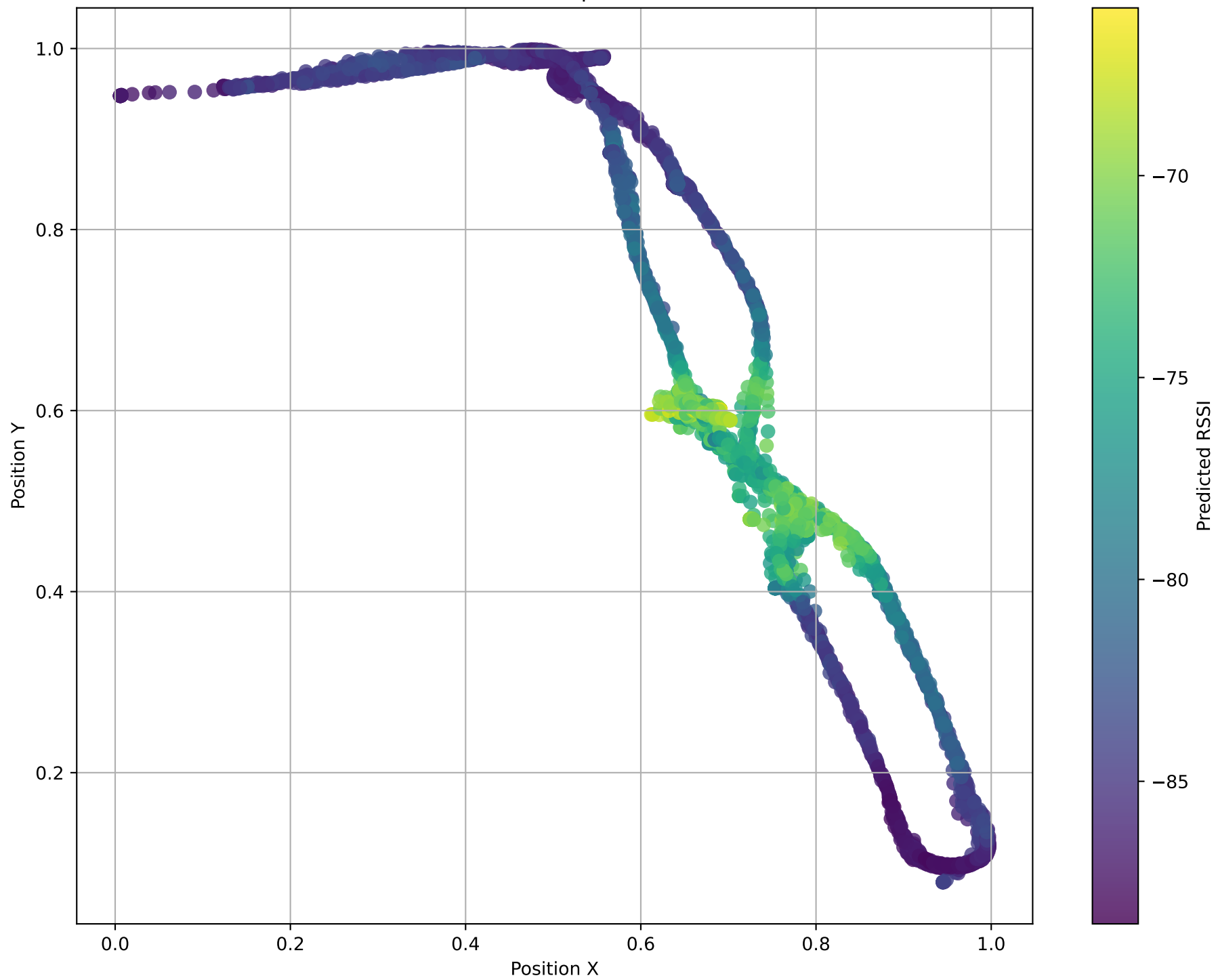
Predicted RSSI in Spatial Context
