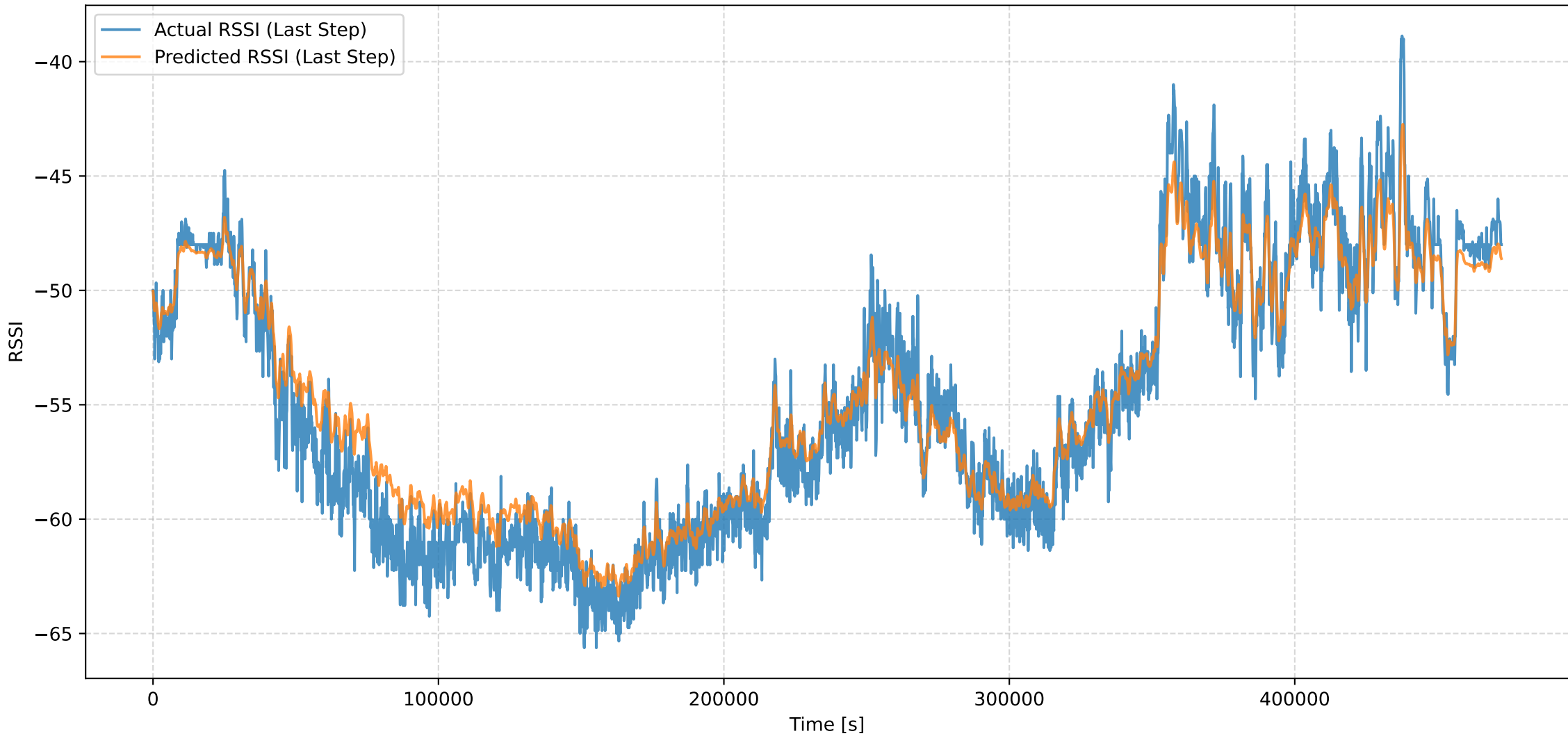
Actual vs Predicted RSSI (Last Step - step 30 \approx 3.0s) [lag=33 samples \approx 3.30s]
