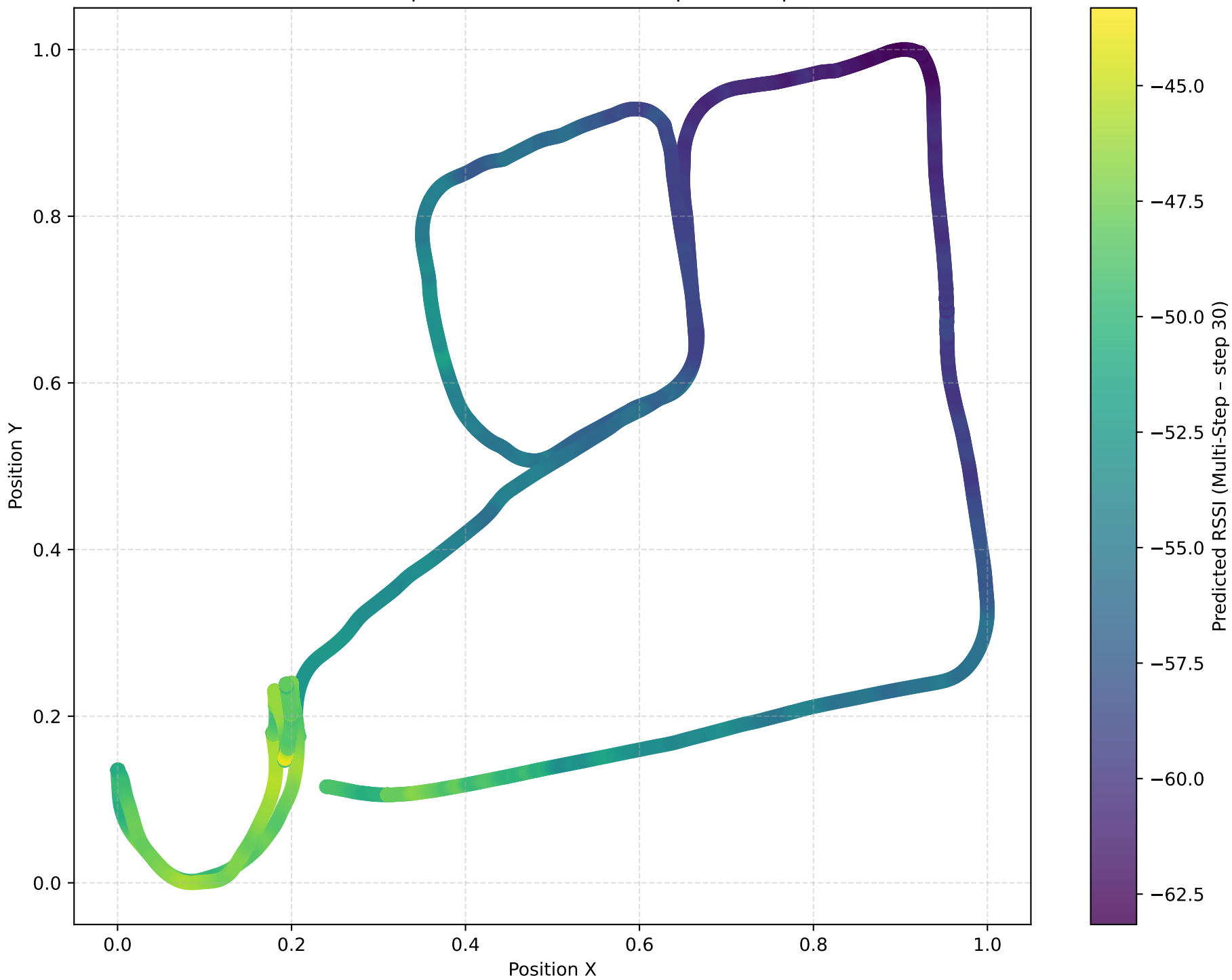
Predicted RSSI in Spatial Context (Multi-Step - 30 steps \approx 3.0 s)
