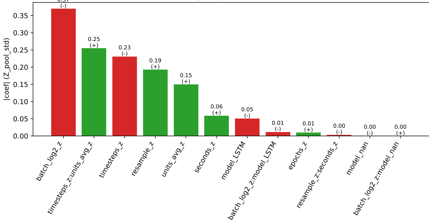
Pareto |coef| - B→A ( R^2 \approx 0.291 )
