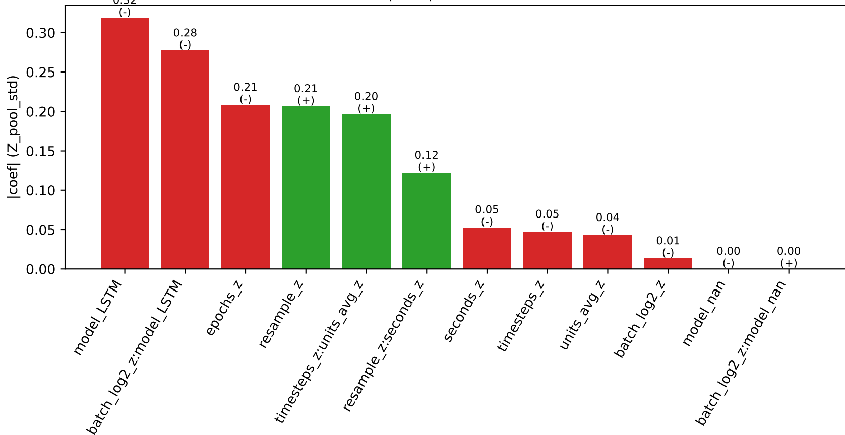
Pareto |coef| - A→B ( R^2 \approx 0.231 )
