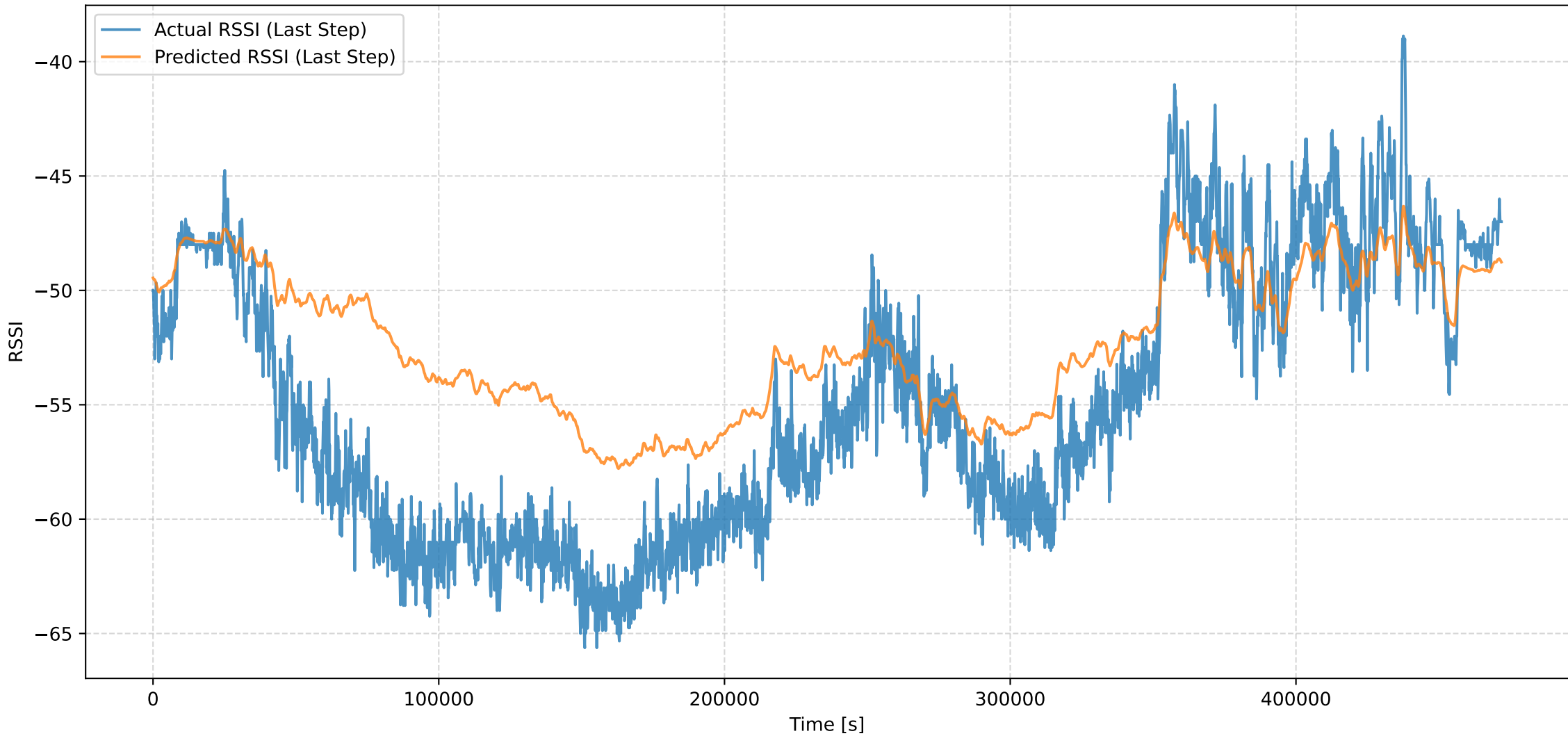
Actual vs Predicted RSSI (Last Step - step 30 \approx 3.0s) [lag=38 samples \approx 3.80s]
