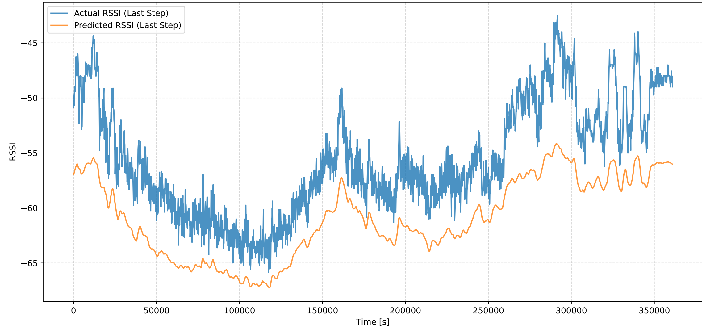
Actual vs Predicted RSSI (Last Step - step 30 \approx 3.0s) [lag=39 samples \approx 3.90s]
