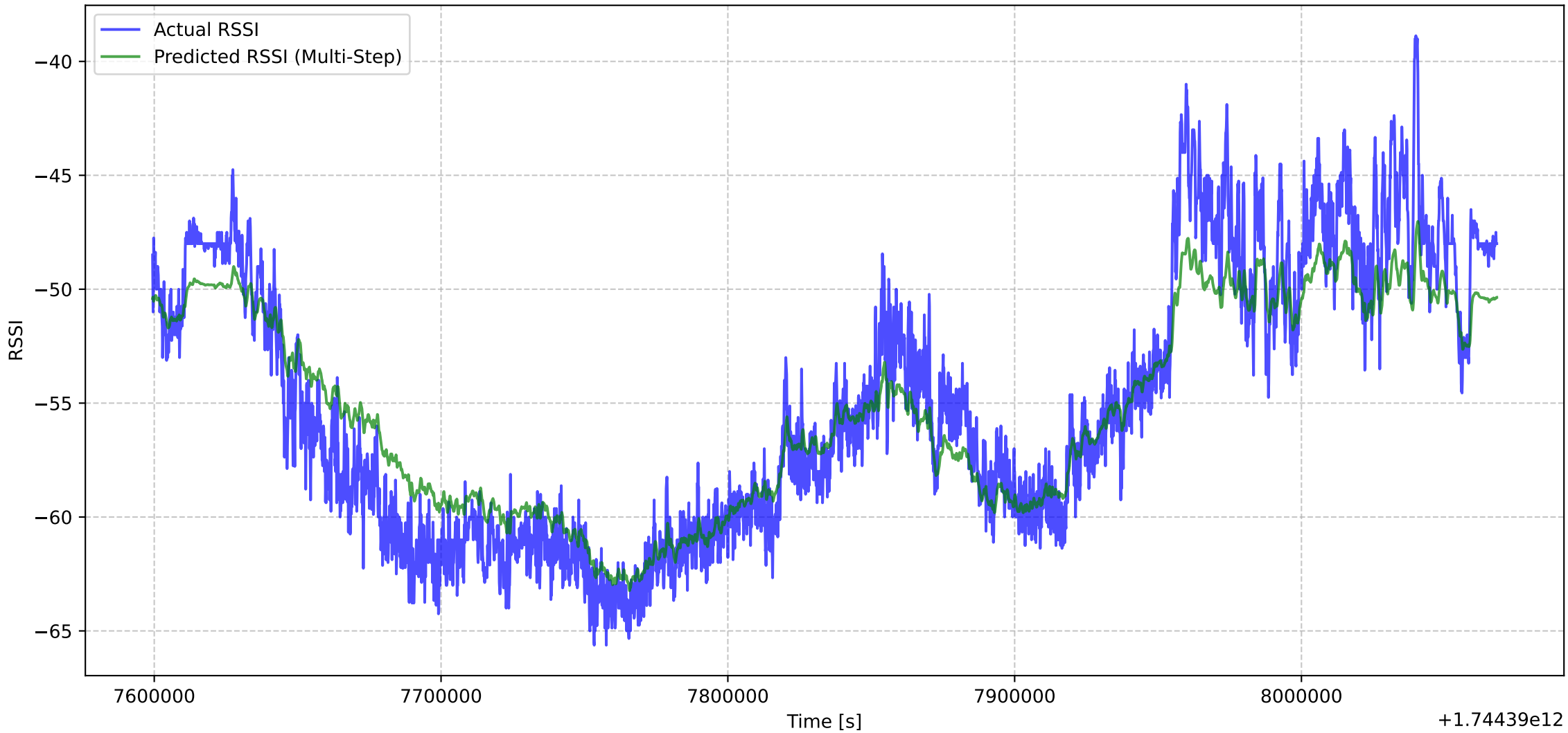
Actual vs Predicted RSSI (Multi-Step (step 100 \approx 10.0 s))
