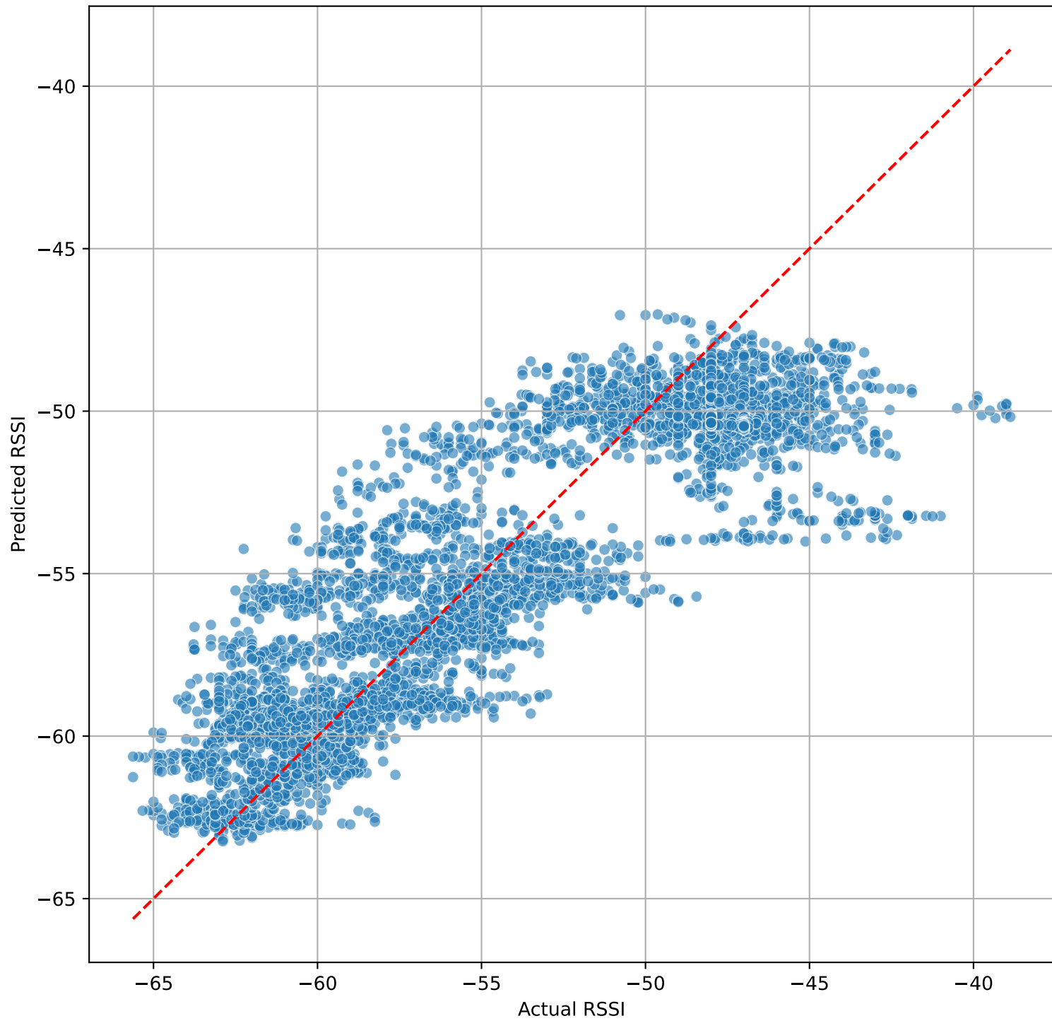
Actual vs Predicted RSSI (Last Step - step 100 \approx 10.0 s)
