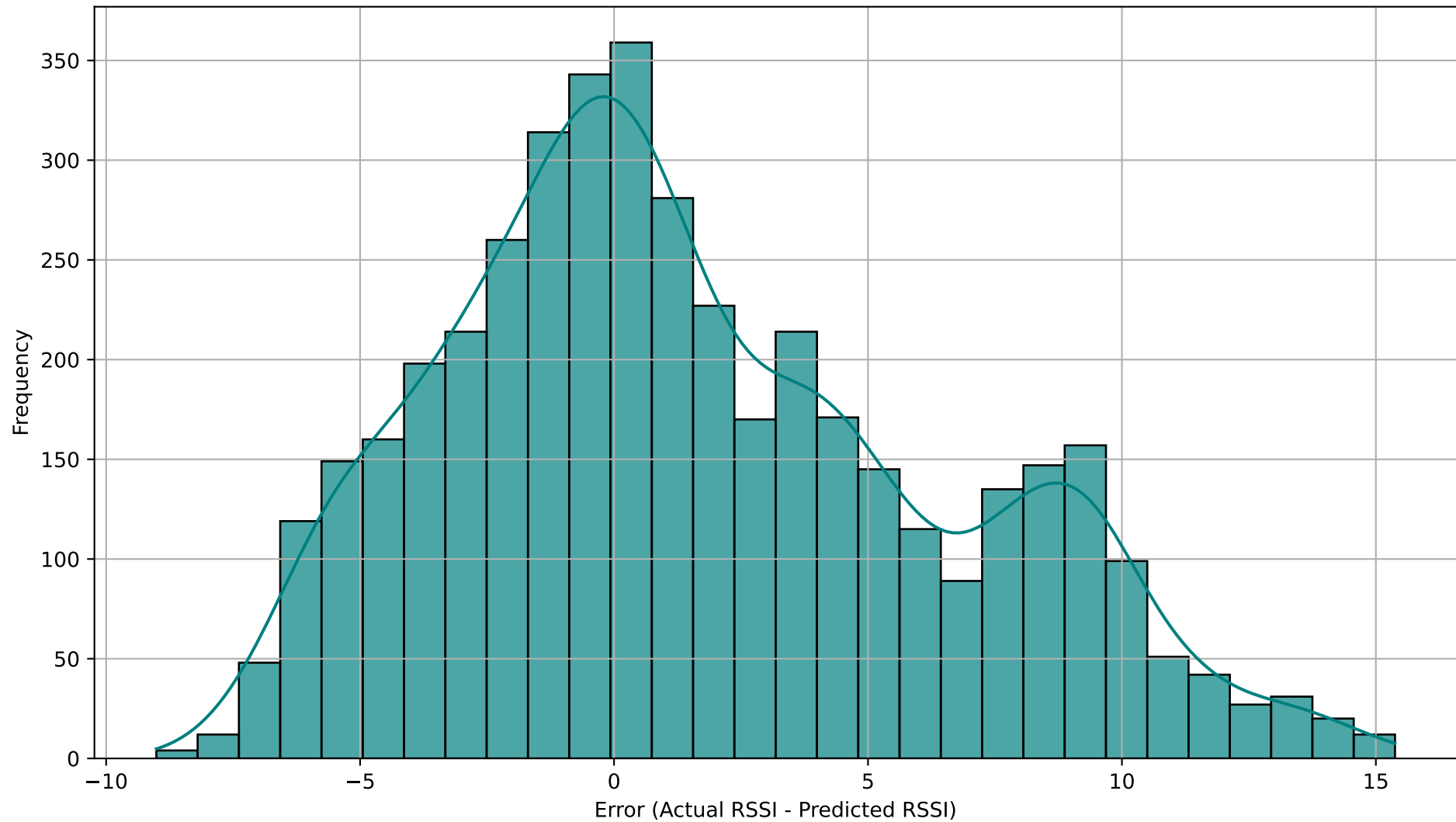
Distribution of Prediction Errors (Last Step - step 300 \approx 25.0 s)
