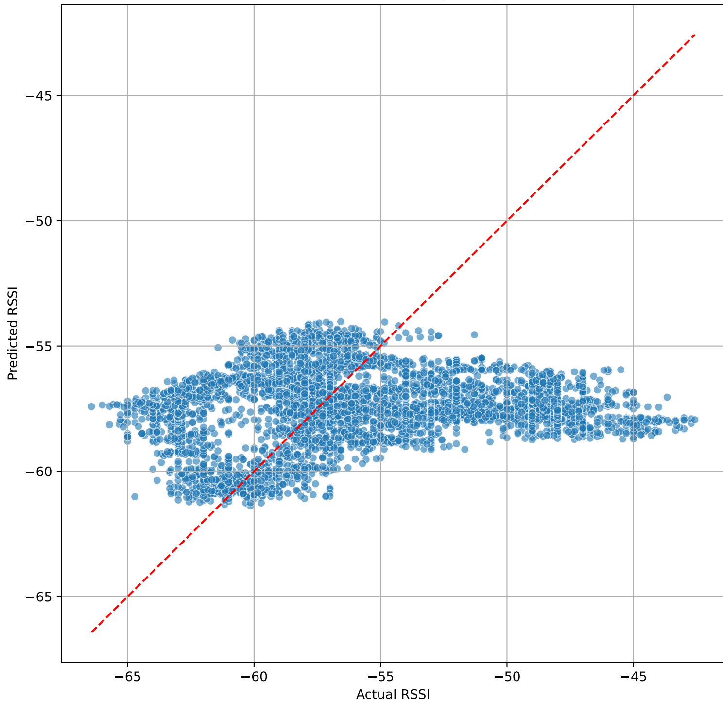
Actual vs Predicted RSSI (Last Step - step 300 \approx 25.0 s)
