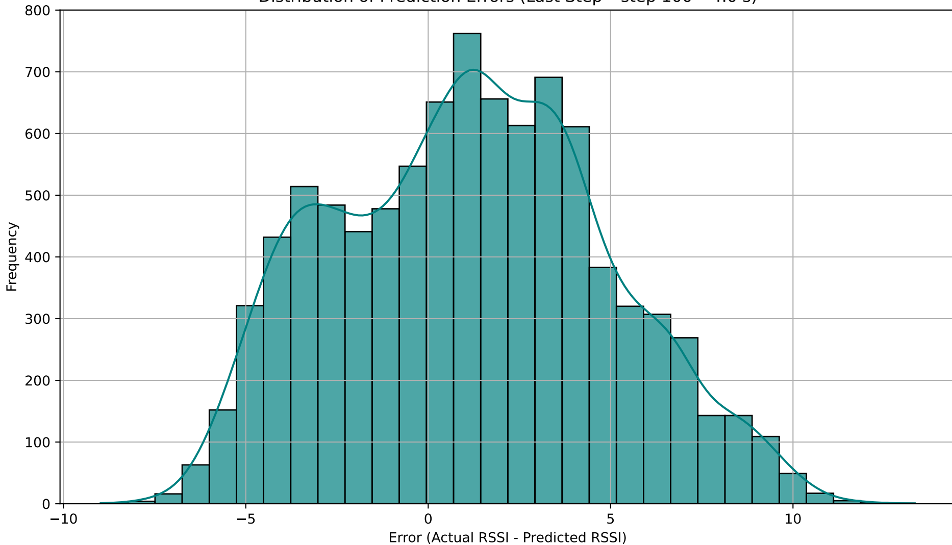
Distribution of Prediction Errors (Last Step - step 100 \approx 4.0 s)
