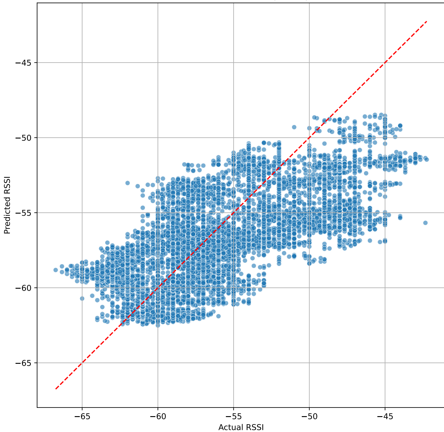
Actual vs Predicted RSSI (Last Step - step 100 \approx 4.0 s)
