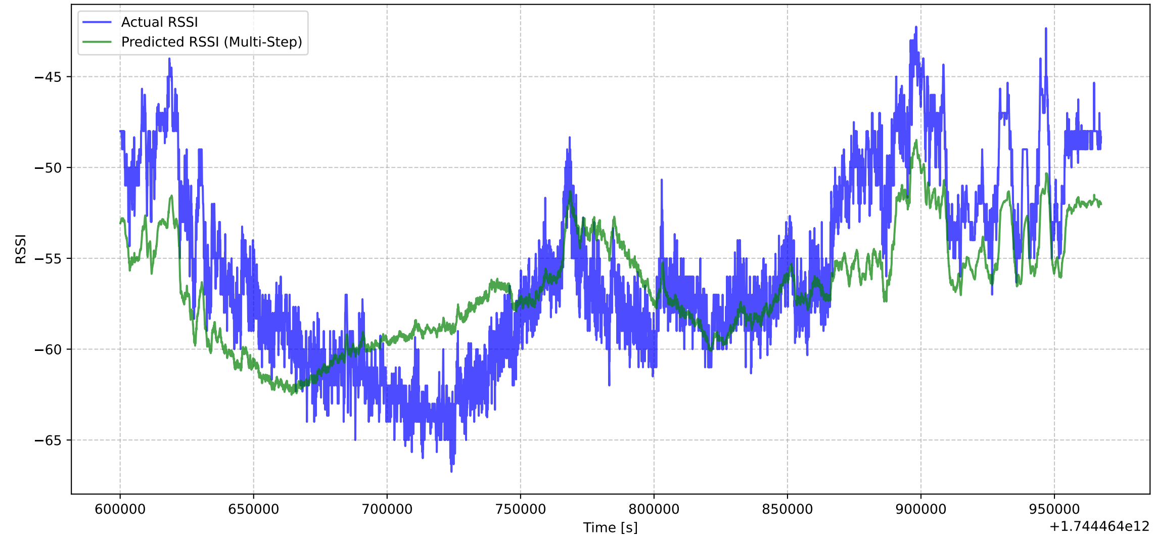
Actual vs Predicted RSSI (Multi-Step (step 100 \approx 4.0 s))
